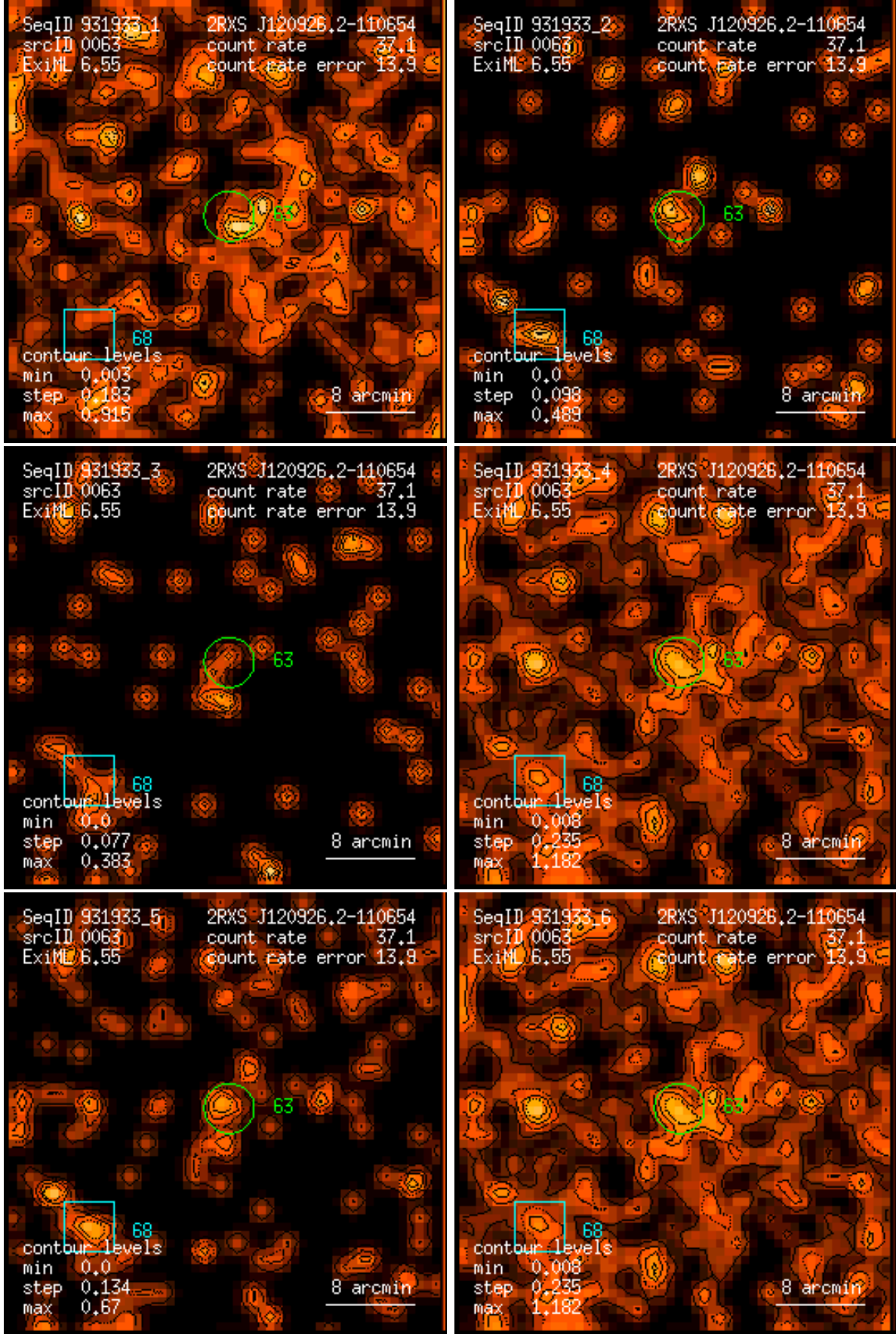
Figure 63: RASS 931933: detection 0063: band rate images, Gaussian filter: (1) PSPC channels 11 – 41, (2) 52 – 90, (3) 91 – 201, (4) 11 – 235, (5) 52 – 201, (6) 11 – 201. Broad band rates in counts/ks. Band rate contour levels in counts/ks/arcmin 2 .
