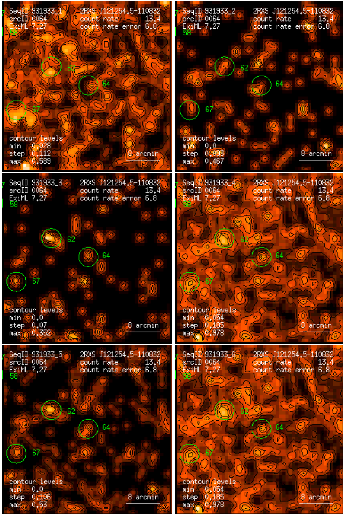
Figure 64: RASS 931933: detection 0064: band rate images, Gaussian filter: (1) PSPC channels 11 – 41, (2) 52 – 90, (3) 91 – 201, (4) 11 – 235, (5) 52 – 201, (6) 11 – 201. Broad band rates in counts/ks. Band rate contour levels in counts/ks/arcmin 2 .
