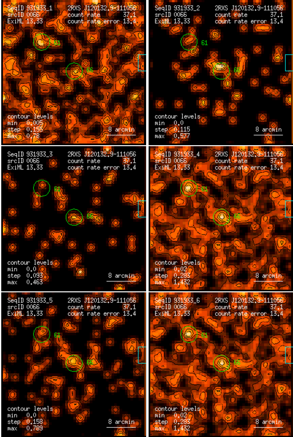
Figure 66: RASS 931933: detection 0066: band rate images, Gaussian filter: (1) PSPC channels 11 – 41, (2) 52 – 90, (3) 91 – 201, (4) 11 – 235, (5) 52 – 201, (6) 11 – 201. Broad band rates in counts/ks. Band rate contour levels in counts/ks/arcmin 2 .
