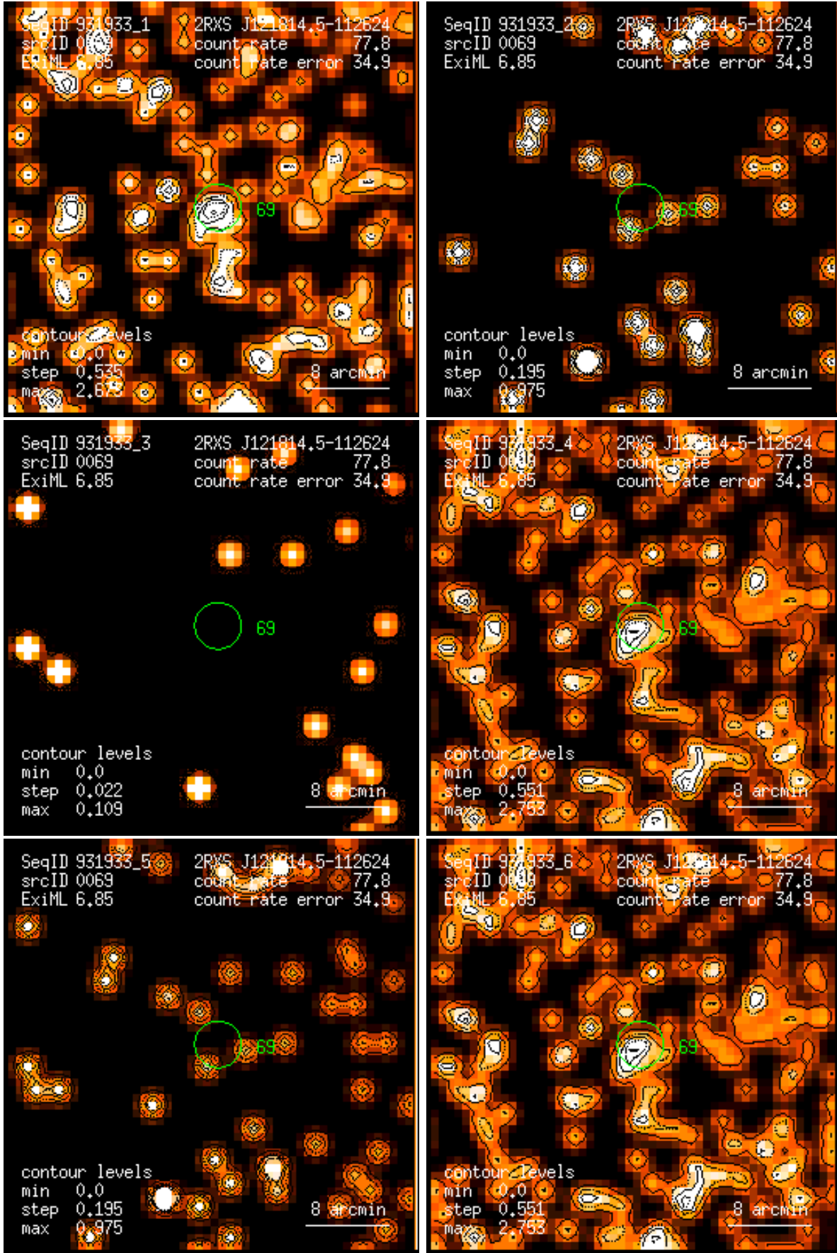
Figure 69: RASS 931933: detection 0069: band rate images, Gaussian filter: (1) PSPC channels 11 – 41, (2) 52 – 90, (3) 91 – 201, (4) 11 – 235, (5) 52 – 201, (6) 11 – 201. Broad band rates in counts/ks. Band rate contour levels in counts/ks/arcmin 2 .
