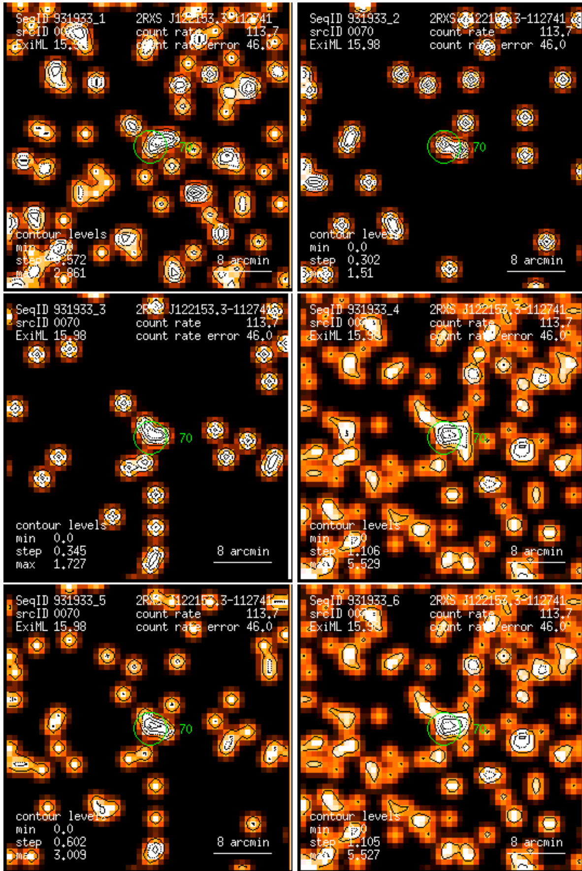
Figure 70: RASS 931933: detection 0070: band rate images, Gaussian filter: (1) PSPC channels 11 – 41, (2) 52 – 90, (3) 91 – 201, (4) 11 – 235, (5) 52 – 201, (6) 11 – 201. Broad band rates in counts/ks. Band rate contour levels in counts/ks/arcmin 2 .
