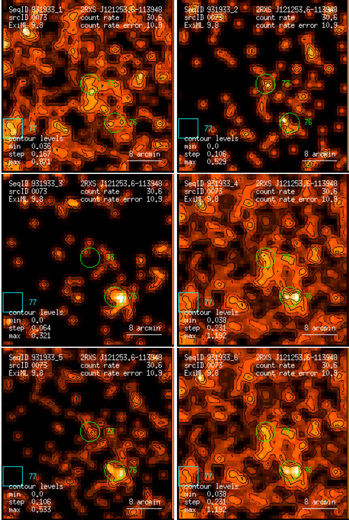
Figure 73: RASS 931933: detection 0073: band rate images, Gaussian filter: (1) PSPC channels 11 – 41, (2) 52 – 90, (3) 91 – 201, (4) 11 – 235, (5) 52 – 201, (6) 11 – 201. Broad band rates in counts/ks. Band rate contour levels in counts/ks/arcmin 2 .
