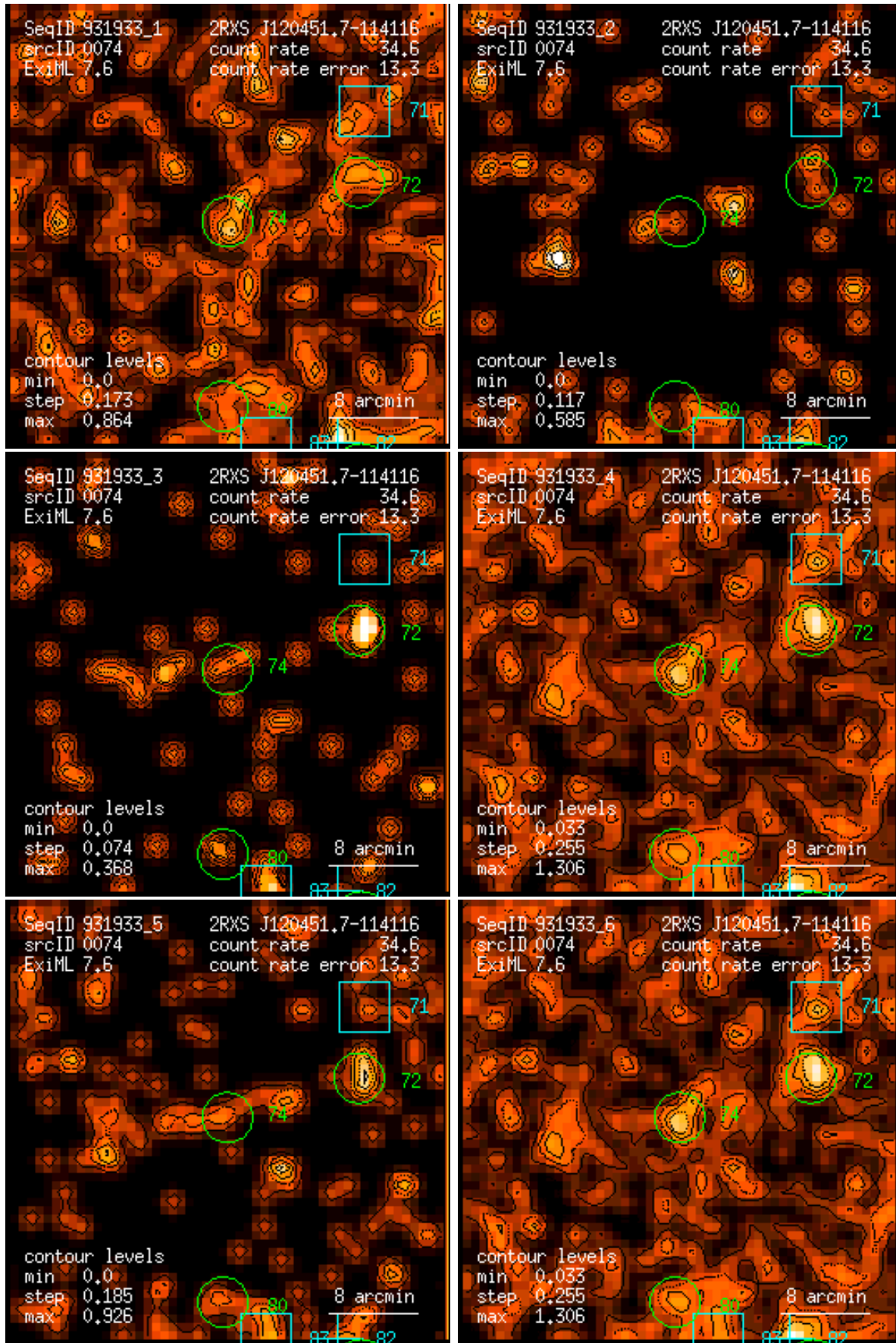
Figure 74: RASS 931933: detection 0074: band rate images, Gaussian filter: (1) PSPC channels 11 – 41, (2) 52 – 90, (3) 91 – 201, (4) 11 – 235, (5) 52 – 201, (6) 11 – 201. Broad band rates in counts/ks. Band rate contour levels in counts/ks/arcmin 2 .
