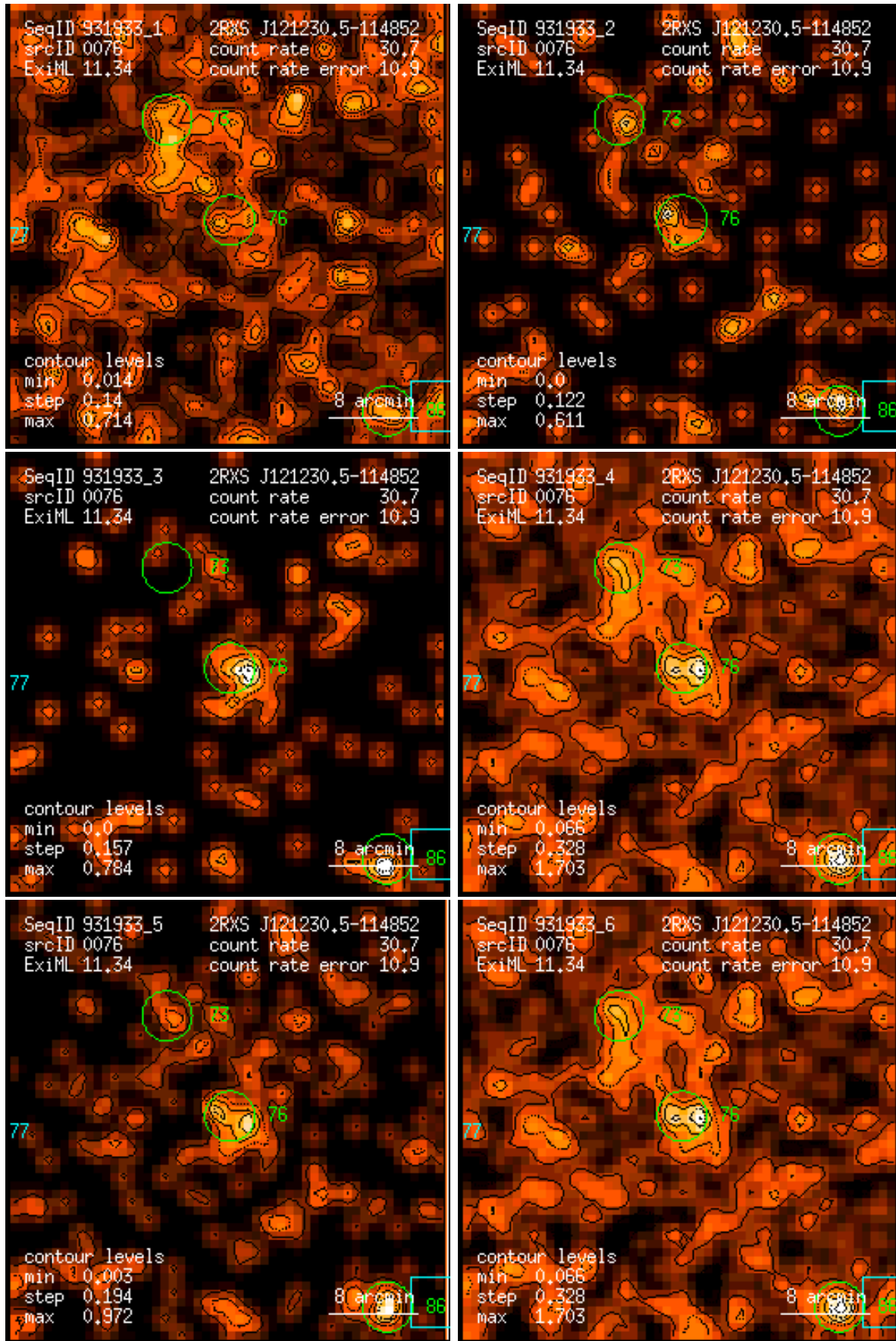
Figure 76: RASS 931933: detection 0076: band rate images, Gaussian filter: (1) PSPC channels 11 – 41, (2) 52 – 90, (3) 91 – 201, (4) 11 – 235, (5) 52 – 201, (6) 11 – 201. Broad band rates in counts/ks. Band rate contour levels in counts/ks/arcmin 2 .
