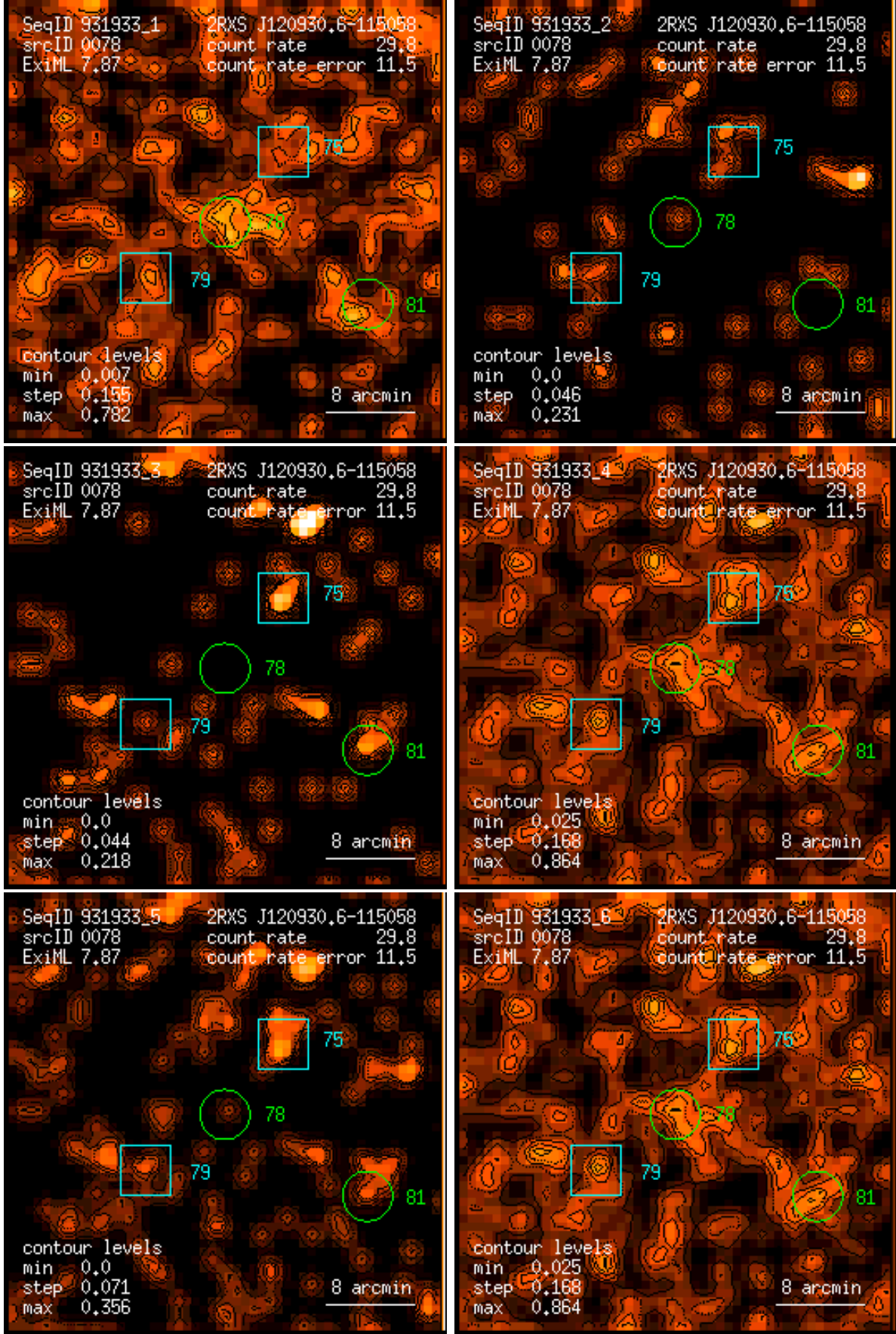
Figure 78: RASS 931933: detection 0078: band rate images, Gaussian filter: (1) PSPC channels 11 – 41, (2) 52 – 90, (3) 91 – 201, (4) 11 – 235, (5) 52 – 201, (6) 11 – 201. Broad band rates in counts/ks. Band rate contour levels in counts/ks/arcmin 2 .
