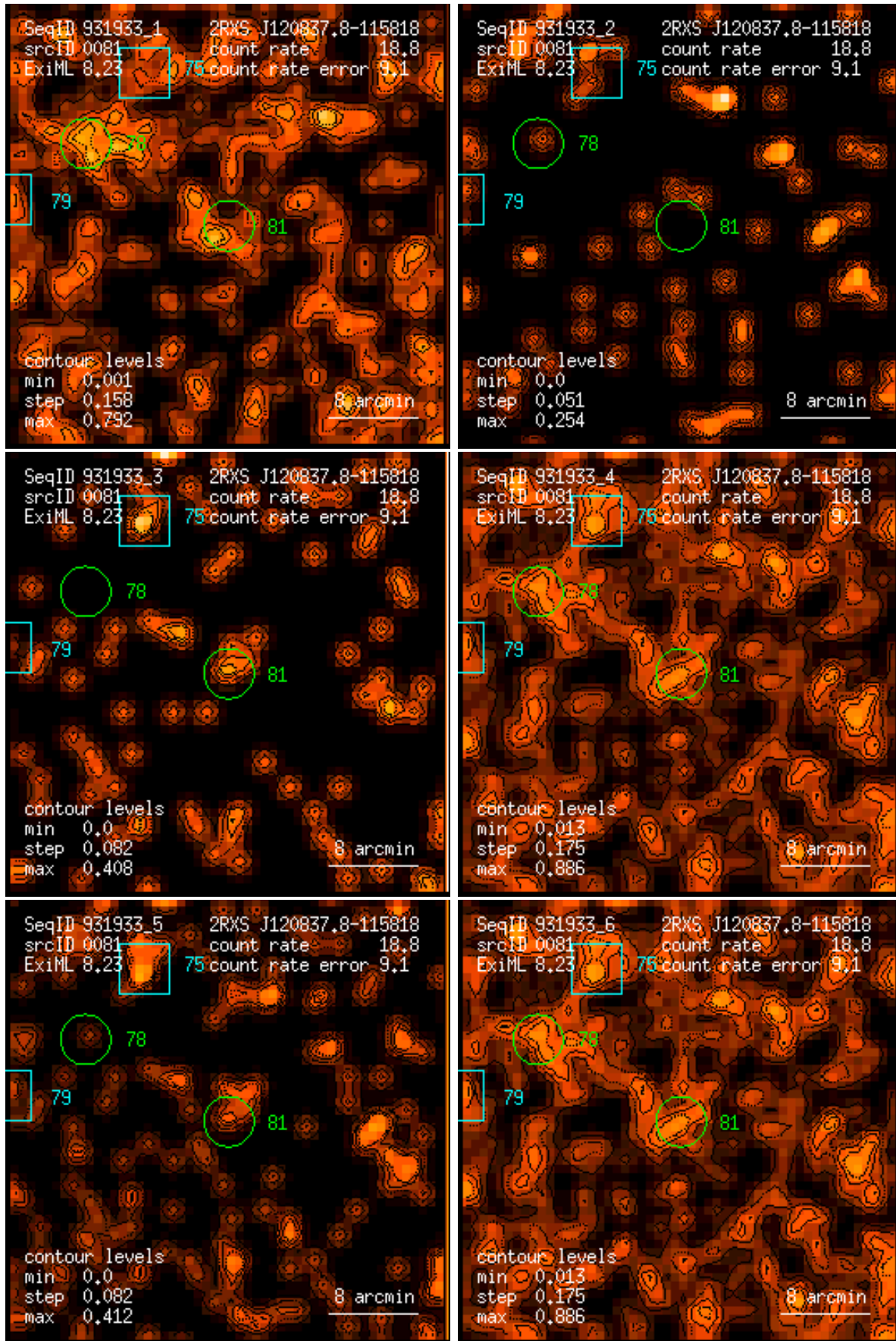
Figure 81: RASS 931933: detection 0081: band rate images, Gaussian filter: (1) PSPC channels 11 – 41, (2) 52 – 90, (3) 91 – 201, (4) 11 – 235, (5) 52 – 201, (6) 11 – 201. Broad band rates in counts/ks. Band rate contour levels in counts/ks/arcmin 2 .
