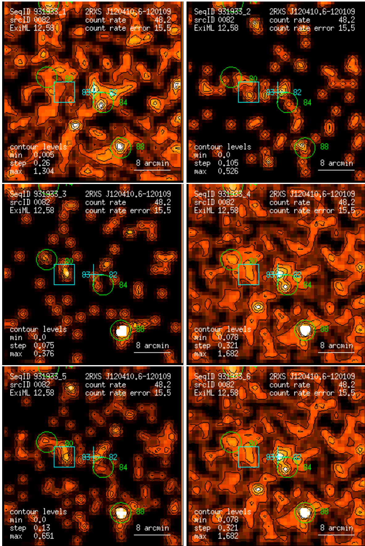
Figure 82: RASS 931933: detection 0082: band rate images, Gaussian filter: (1) PSPC channels 11 – 41, (2) 52 – 90, (3) 91 – 201, (4) 11 – 235, (5) 52 – 201, (6) 11 – 201. Broad band rates in counts/ks. Band rate contour levels in counts/ks/arcmin 2 .
