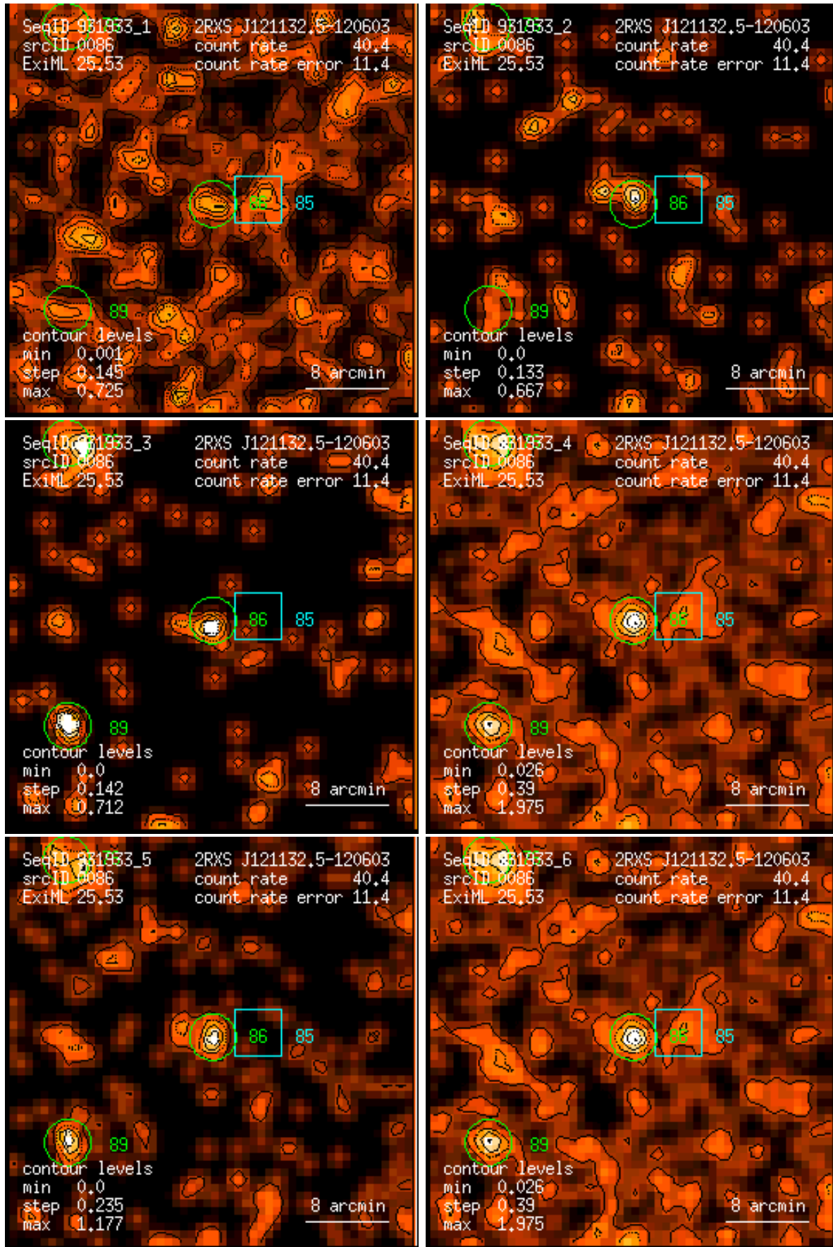
Figure 86: RASS 931933: detection 0086: band rate images, Gaussian filter: (1) PSPC channels 11 – 41, (2) 52 – 90, (3) 91 – 201, (4) 11 – 235, (5) 52 – 201, (6) 11 – 201. Broad band rates in counts/ks. Band rate contour levels in counts/ks/arcmin 2 .
