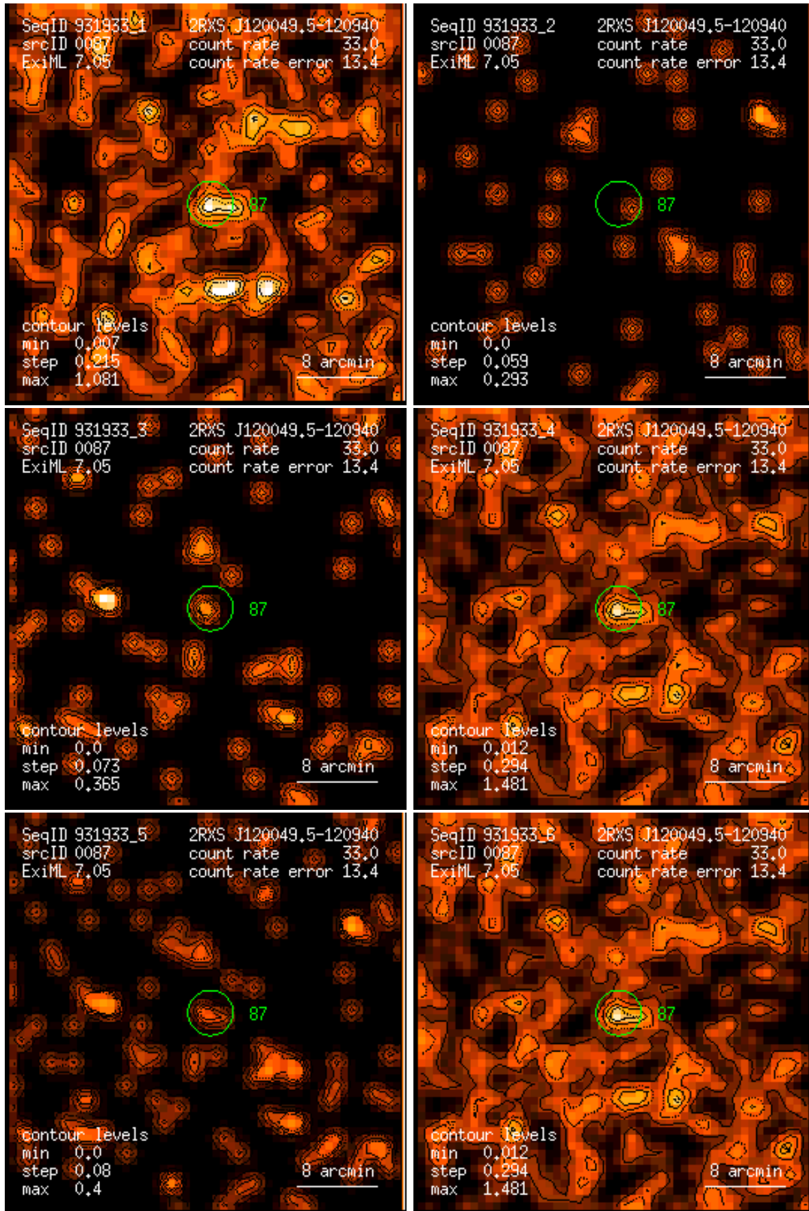
Figure 87: RASS 931933: detection 0087: band rate images, Gaussian filter: (1) PSPC channels 11 – 41, (2) 52 – 90, (3) 91 – 201, (4) 11 – 235, (5) 52 – 201, (6) 11 – 201. Broad band rates in counts/ks. Band rate contour levels in counts/ks/arcmin 2 .
