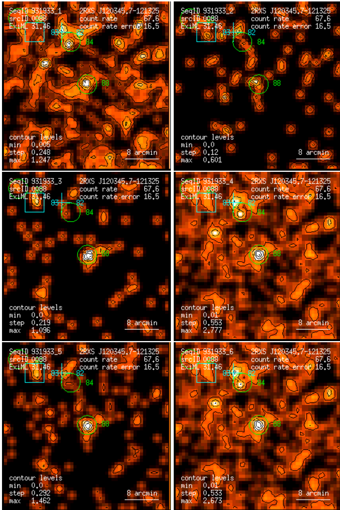
Figure 88: RASS 931933: detection 0088: band rate images, Gaussian filter: (1) PSPC channels 11 – 41, (2) 52 – 90, (3) 91 – 201, (4) 11 – 235, (5) 52 – 201, (6) 11 – 201. Broad band rates in counts/ks. Band rate contour levels in counts/ks/arcmin 2 .
