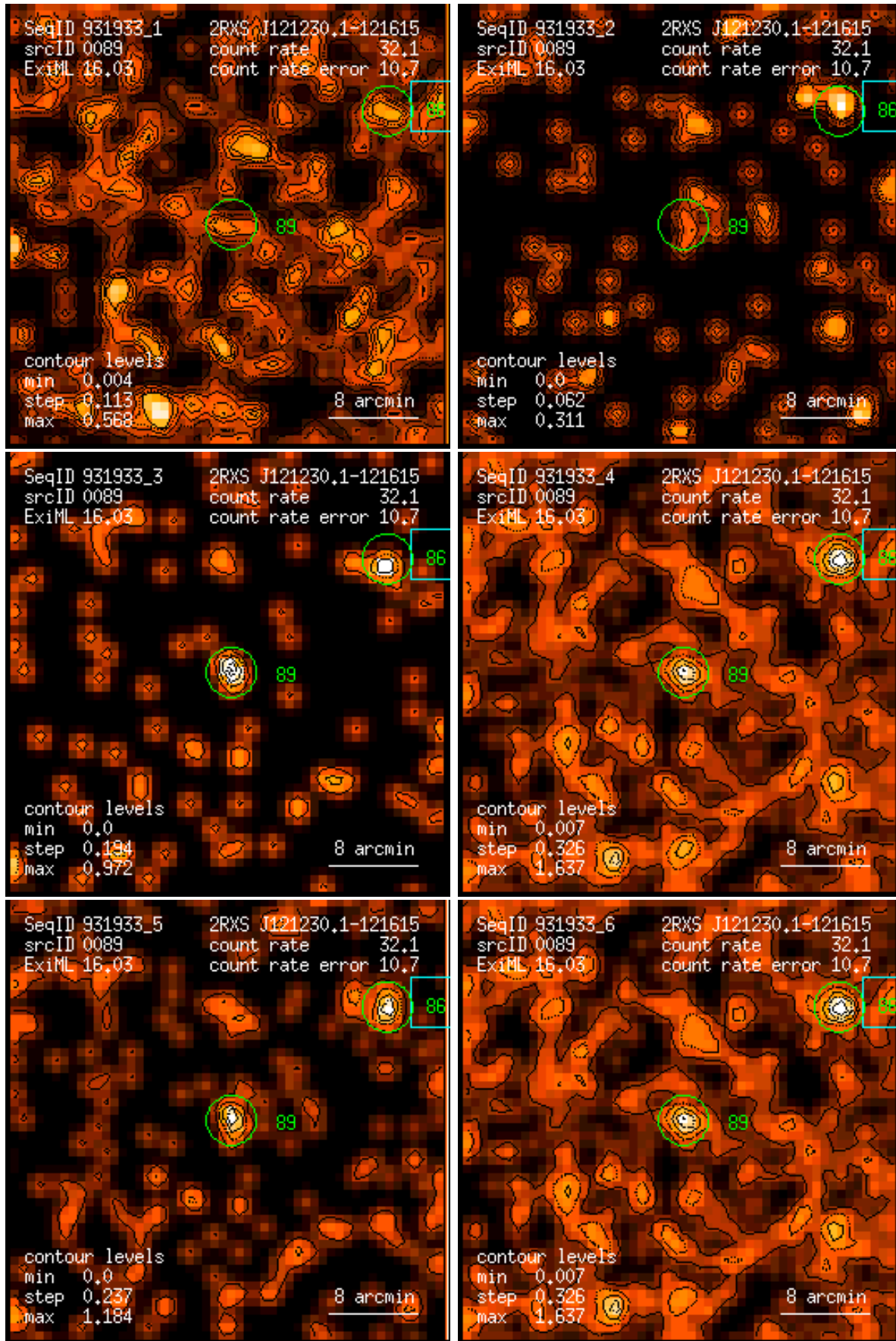
Figure 89: RASS 931933: detection 0089: band rate images, Gaussian filter: (1) PSPC channels 11 – 41, (2) 52 – 90, (3) 91 – 201, (4) 11 – 235, (5) 52 – 201, (6) 11 – 201. Broad band rates in counts/ks. Band rate contour levels in counts/ks/arcmin 2 .
