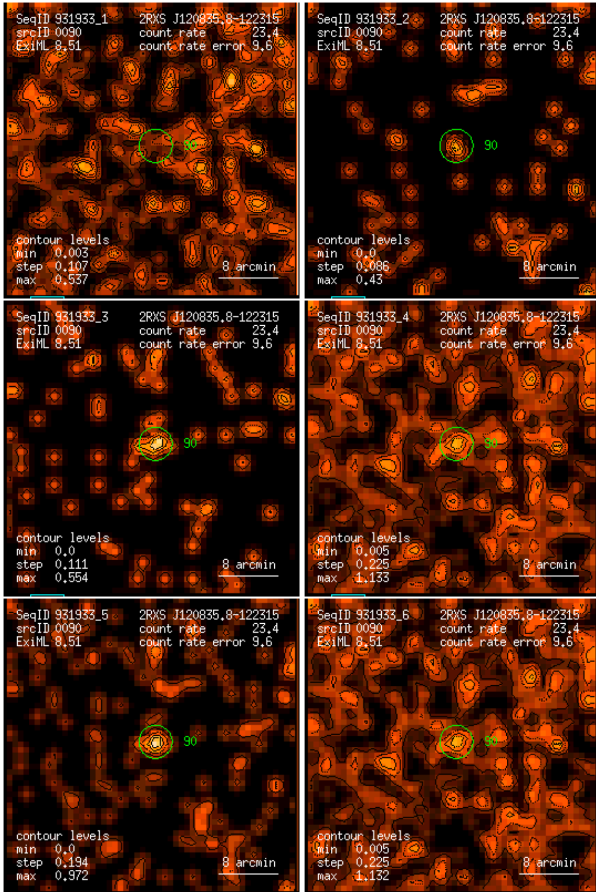
Figure 90: RASS 931933: detection 0090: band rate images, Gaussian filter: (1) PSPC channels 11 – 41, (2) 52 – 90, (3) 91 – 201, (4) 11 – 235, (5) 52 – 201, (6) 11 – 201. Broad band rates in counts/ks. Band rate contour levels in counts/ks/arcmin 2 .
