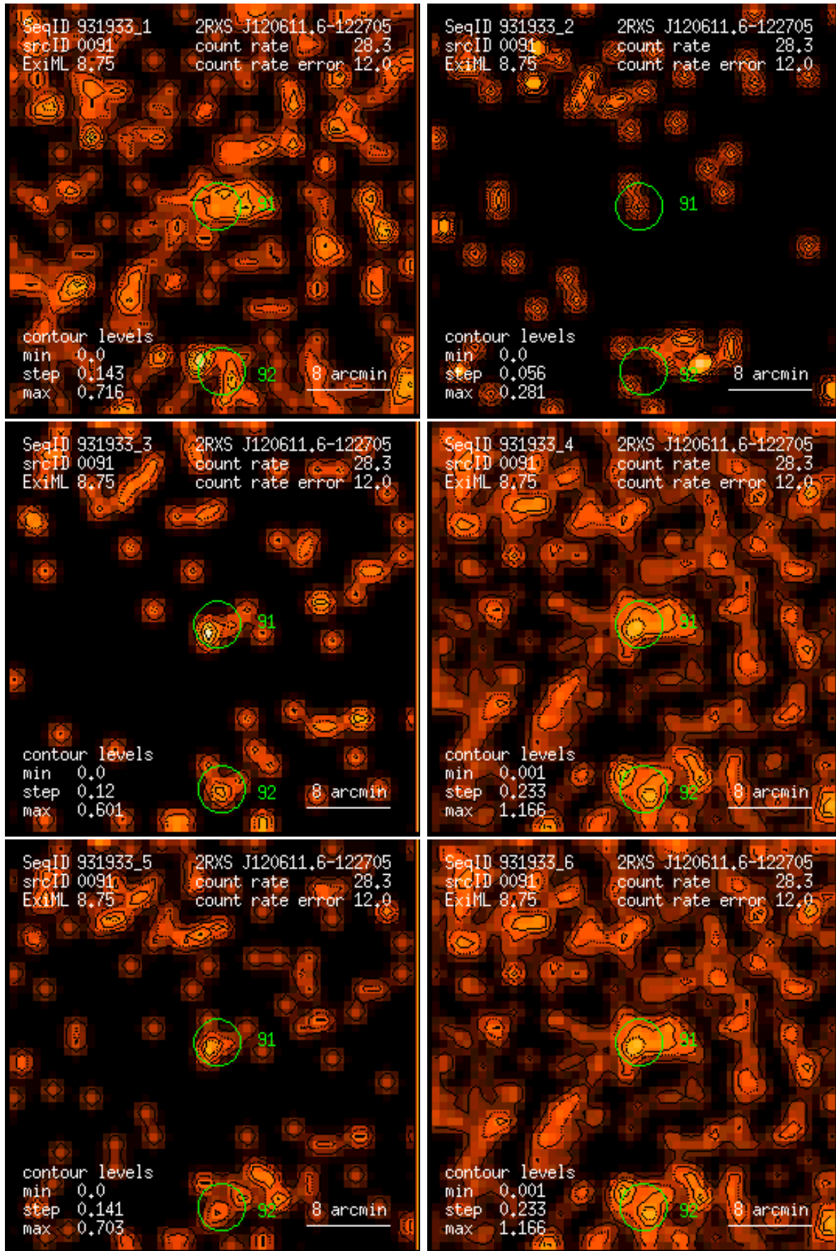
Figure 91: RASS 931933: detection 0091: band rate images, Gaussian filter: (1) PSPC channels 11 – 41, (2) 52 – 90, (3) 91 – 201, (4) 11 – 235, (5) 52 – 201, (6) 11 – 201. Broad band rates in counts/ks. Band rate contour levels in counts/ks/arcmin 2 .
