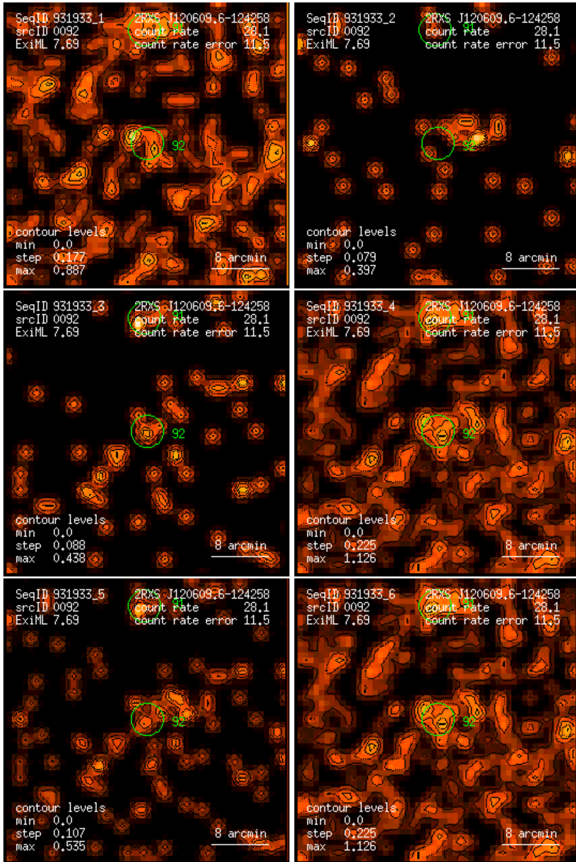
Figure 92: RASS 931933: detection 0092: band rate images, Gaussian filter: (1) PSPC channels 11 – 41, (2) 52 – 90, (3) 91 – 201, (4) 11 – 235, (5) 52 – 201, (6) 11 – 201. Broad band rates in counts/ks. Band rate contour levels in counts/ks/arcmin 2 .
