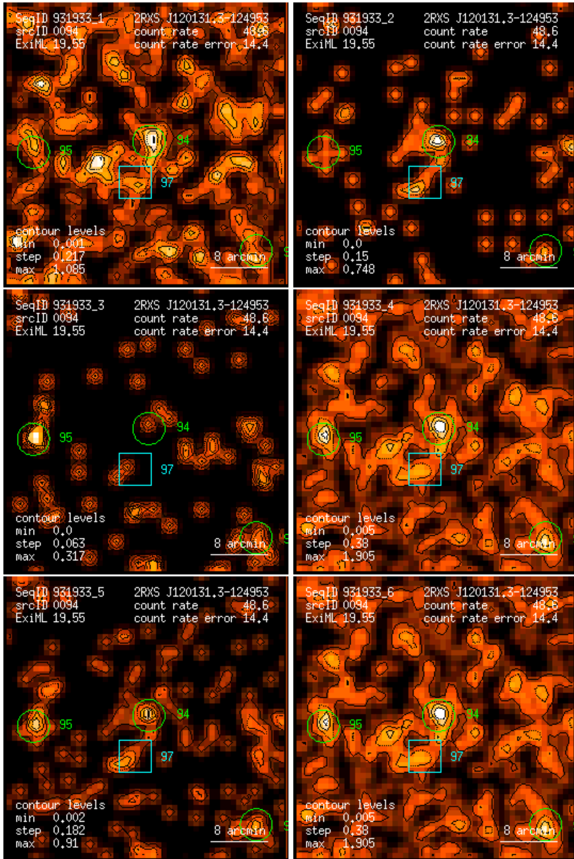
Figure 94: RASS 931933: detection 0094: band rate images, Gaussian filter: (1) PSPC channels 11 – 41, (2) 52 – 90, (3) 91 – 201, (4) 11 – 235, (5) 52 – 201, (6) 11 – 201. Broad band rates in counts/ks. Band rate contour levels in counts/ks/arcmin 2 .
