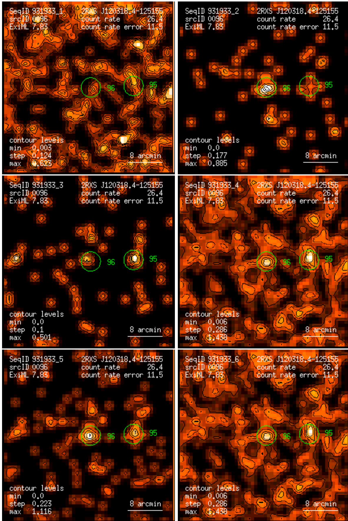
Figure 96: RASS 931933: detection 0096: band rate images, Gaussian filter: (1) PSPC channels 11 – 41, (2) 52 – 90, (3) 91 – 201, (4) 11 – 235, (5) 52 – 201, (6) 11 – 201. Broad band rates in counts/ks. Band rate contour levels in counts/ks/arcmin 2 .
