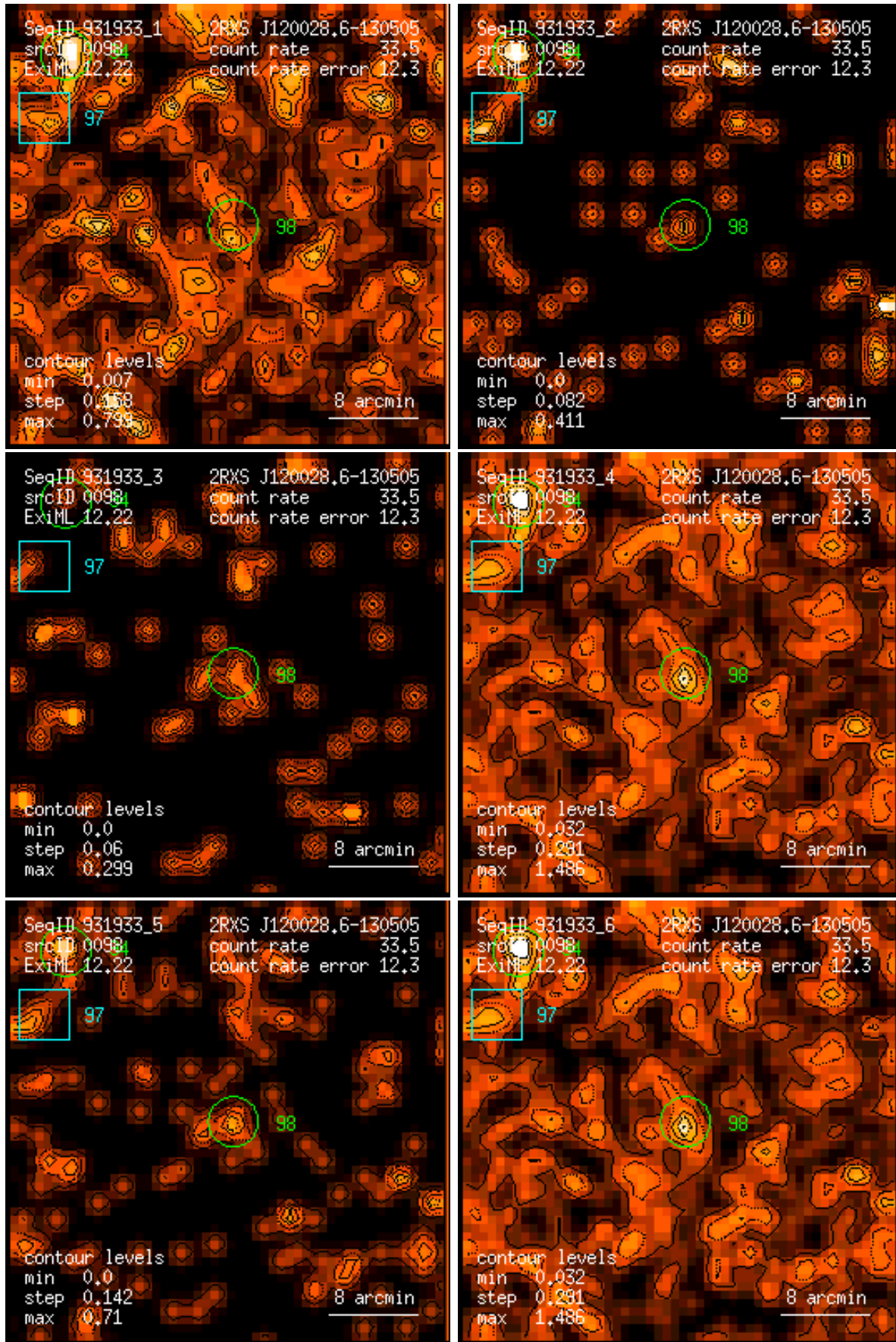
Figure 98: RASS 931933: detection 0098: band rate images, Gaussian filter: (1) PSPC channels 11 – 41, (2) 52 – 90, (3) 91 – 201, (4) 11 – 235, (5) 52 – 201, (6) 11 – 201. Broad band rates in counts/ks. Band rate contour levels in counts/ks/arcmin 2 .
