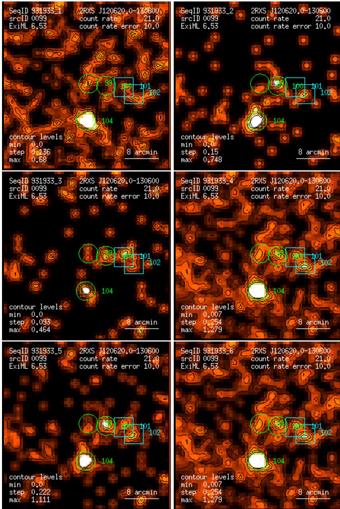
Figure 99: RASS 931933: detection 0099: band rate images, Gaussian filter: (1) PSPC channels 11 – 41, (2) 52 – 90, (3) 91 – 201, (4) 11 – 235, (5) 52 – 201, (6) 11 – 201. Broad band rates in counts/ks. Band rate contour levels in counts/ks/arcmin 2 .
