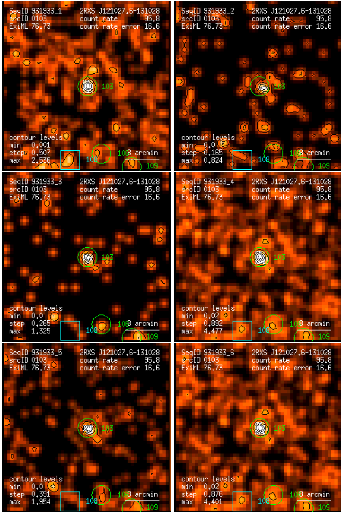
Figure 103: RASS 931933: detection 0103: band rate images, Gaussian filter: (1) PSPC channels 11 – 41, (2) 52 – 90, (3) 91 – 201, (4) 11 – 235, (5) 52 – 201, (6) 11 – 201. Broad band rates in counts/ks. Band rate contour levels in counts/ks/arcmin 2 .
