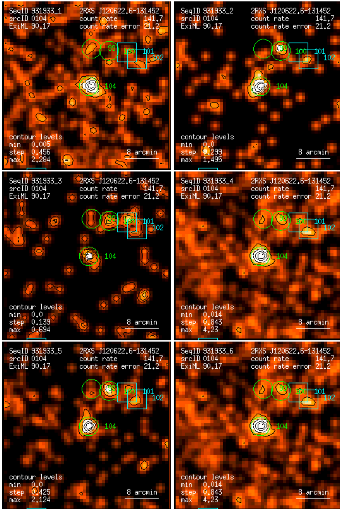
Figure 104: RASS 931933: detection 0104: band rate images, Gaussian filter: (1) PSPC channels 11 – 41, (2) 52 – 90, (3) 91 – 201, (4) 11 – 235, (5) 52 – 201, (6) 11 – 201. Broad band rates in counts/ks. Band rate contour levels in counts/ks/arcmin 2 .
