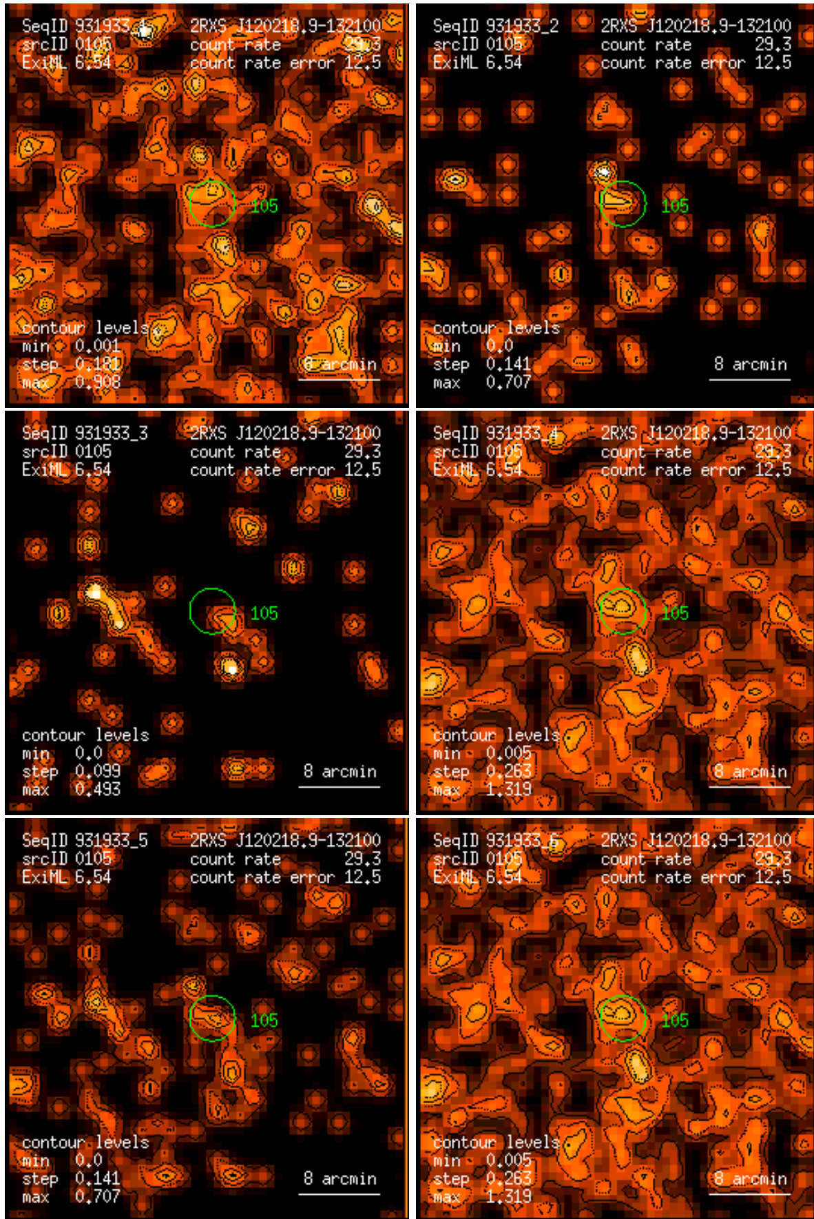
Figure 105: RASS 931933: detection 0105: band rate images, Gaussian filter: (1) PSPC channels 11 – 41, (2) 52 – 90, (3) 91 – 201, (4) 11 – 235, (5) 52 – 201, (6) 11 – 201. Broad band rates in counts/ks. Band rate contour levels in counts/ks/arcmin 2 .
