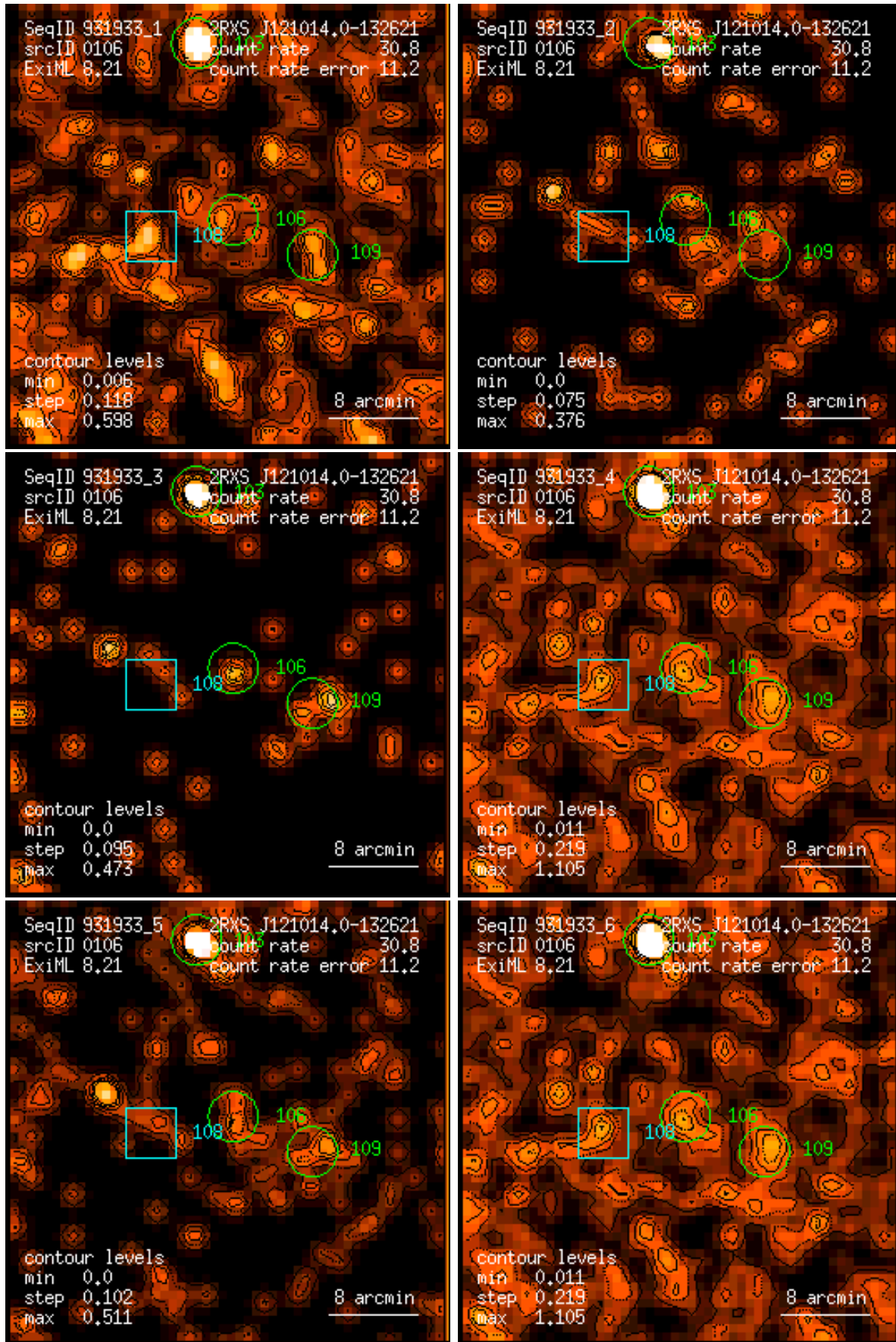
Figure 106: RASS 931933: detection 0106: band rate images, Gaussian filter: (1) PSPC channels 11 – 41, (2) 52 – 90, (3) 91 – 201, (4) 11 – 235, (5) 52 – 201, (6) 11 – 201. Broad band rates in counts/ks. Band rate contour levels in counts/ks/arcmin 2 .
