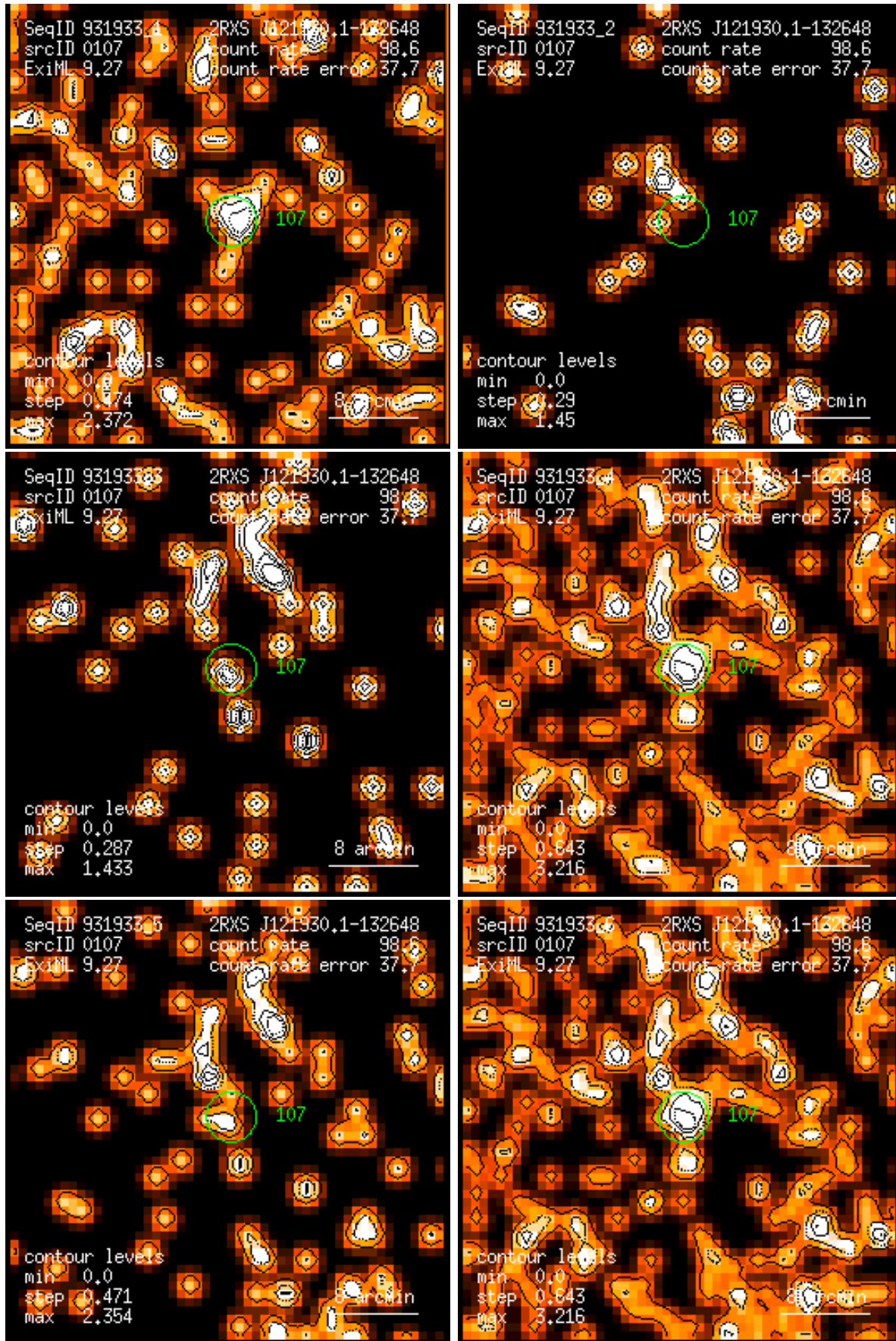
Figure 107: RASS 931933: detection 0107: band rate images, Gaussian filter: (1) PSPC channels 11 – 41, (2) 52 – 90, (3) 91 – 201, (4) 11 – 235, (5) 52 – 201, (6) 11 – 201. Broad band rates in counts/ks. Band rate contour levels in counts/ks/arcmin 2 .
