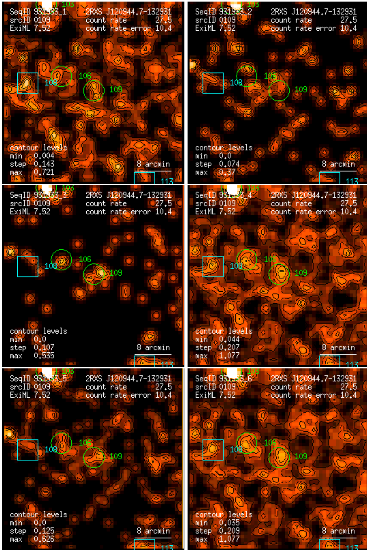
Figure 109: RASS 931933: detection 0109: band rate images, Gaussian filter: (1) PSPC channels 11 – 41, (2) 52 – 90, (3) 91 – 201, (4) 11 – 235, (5) 52 – 201, (6) 11 – 201. Broad band rates in counts/ks. Band rate contour levels in counts/ks/arcmin 2 .
