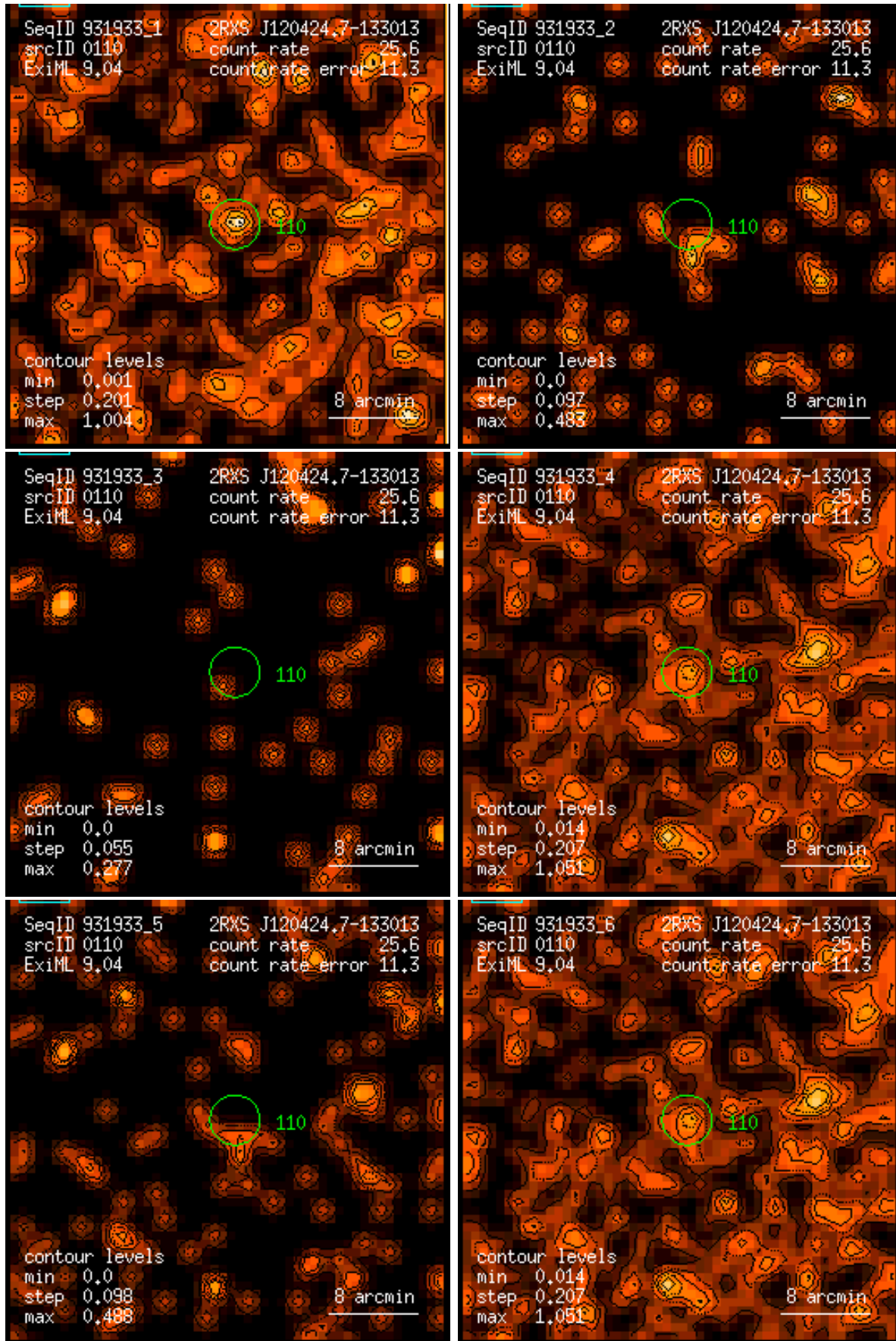
Figure 110: RASS 931933: detection 0110: band rate images, Gaussian filter: (1) PSPC channels 11 – 41, (2) 52 – 90, (3) 91 – 201, (4) 11 – 235, (5) 52 – 201, (6) 11 – 201. Broad band rates in counts/ks. Band rate contour levels in counts/ks/arcmin 2 .
