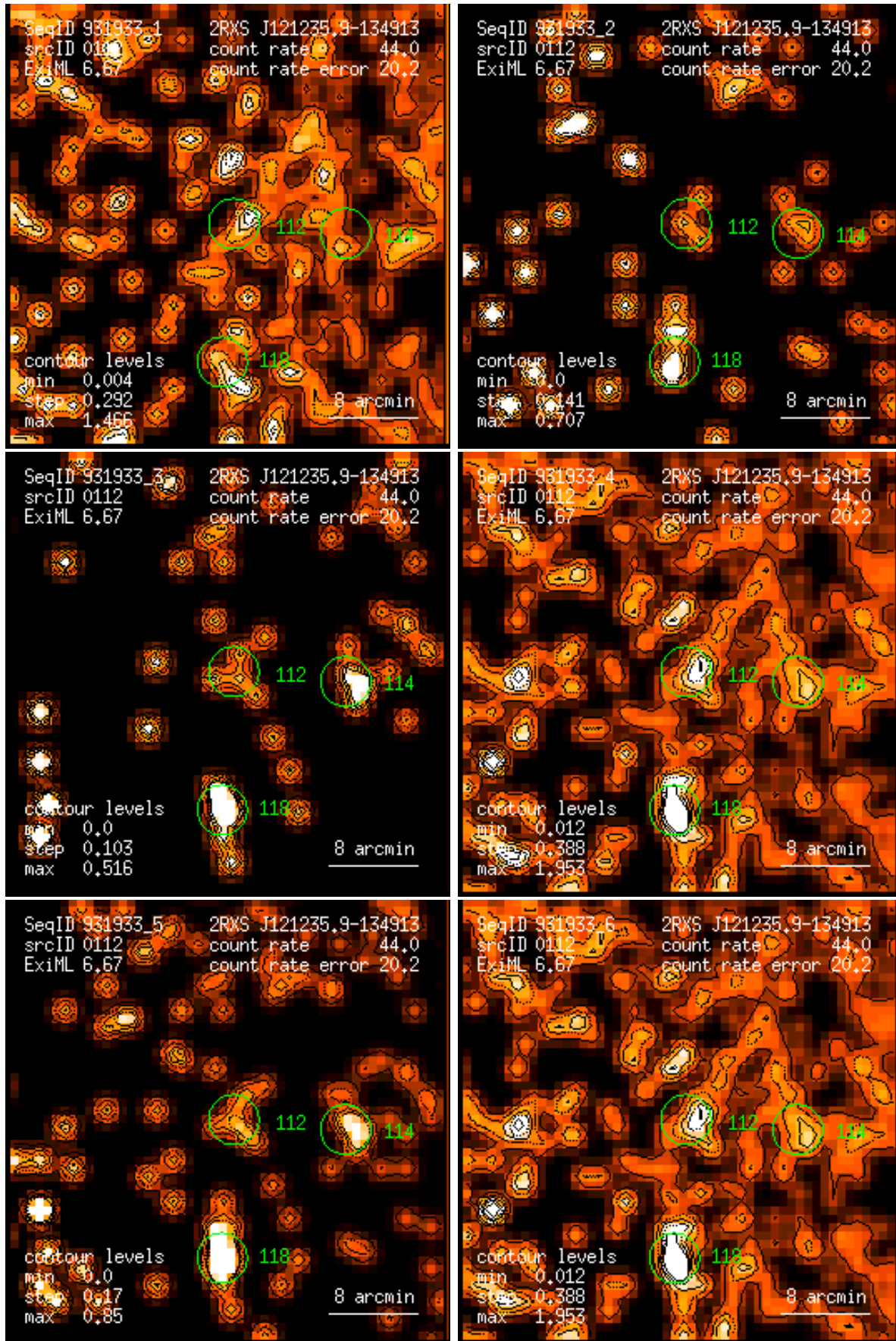
Figure 112: RASS 931933: detection 0112: band rate images, Gaussian filter: (1) PSPC channels 11 – 41, (2) 52 – 90, (3) 91 – 201, (4) 11 – 235, (5) 52 – 201, (6) 11 – 201. Broad band rates in counts/ks. Band rate contour levels in counts/ks/arcmin 2 .
