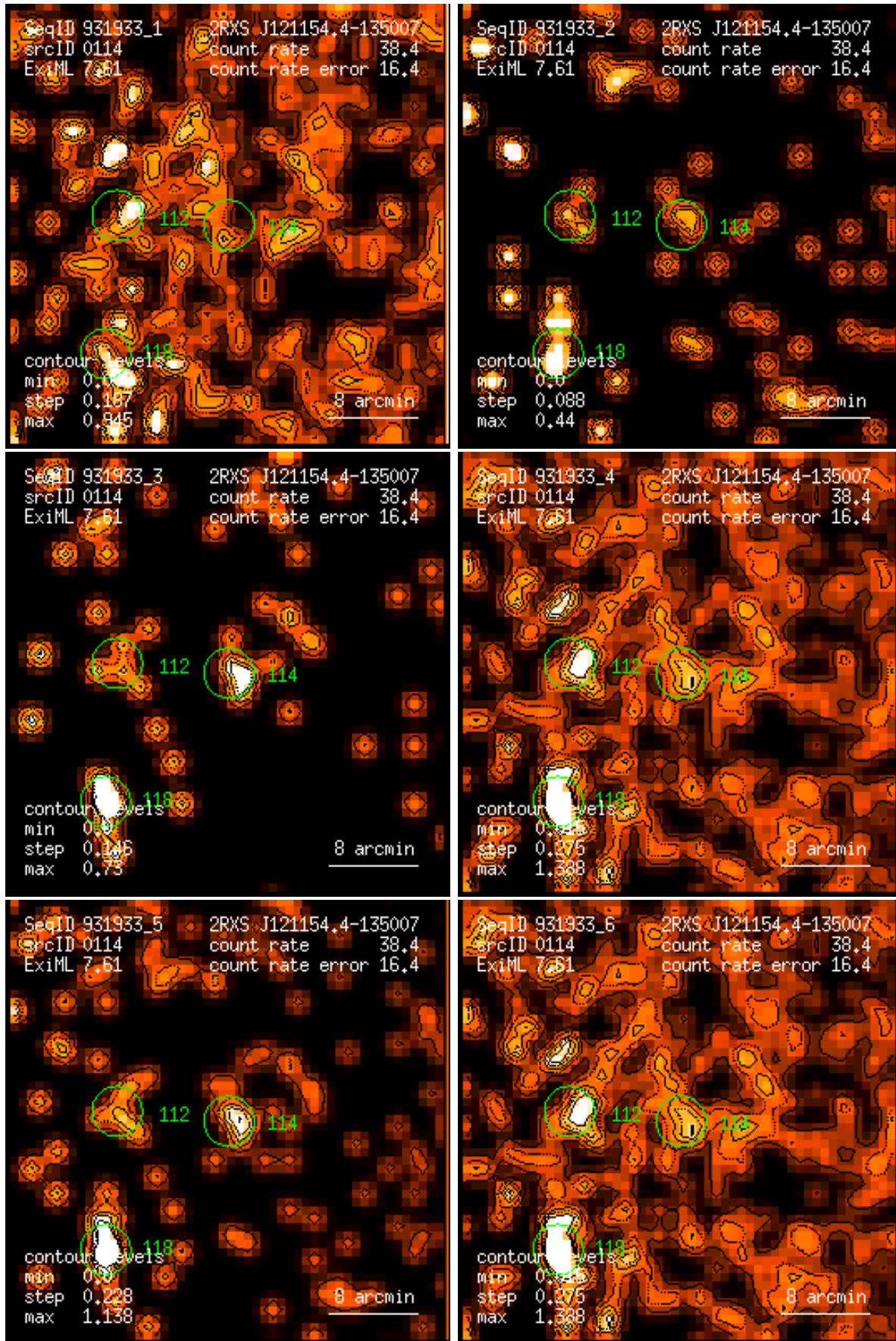
Figure 114: RASS 931933: detection 0114: band rate images, Gaussian filter: (1) PSPC channels 11 – 41, (2) 52 – 90, (3) 91 – 201, (4) 11 – 235, (5) 52 – 201, (6) 11 – 201. Broad band rates in counts/ks. Band rate contour levels in counts/ks/arcmin 2 .
