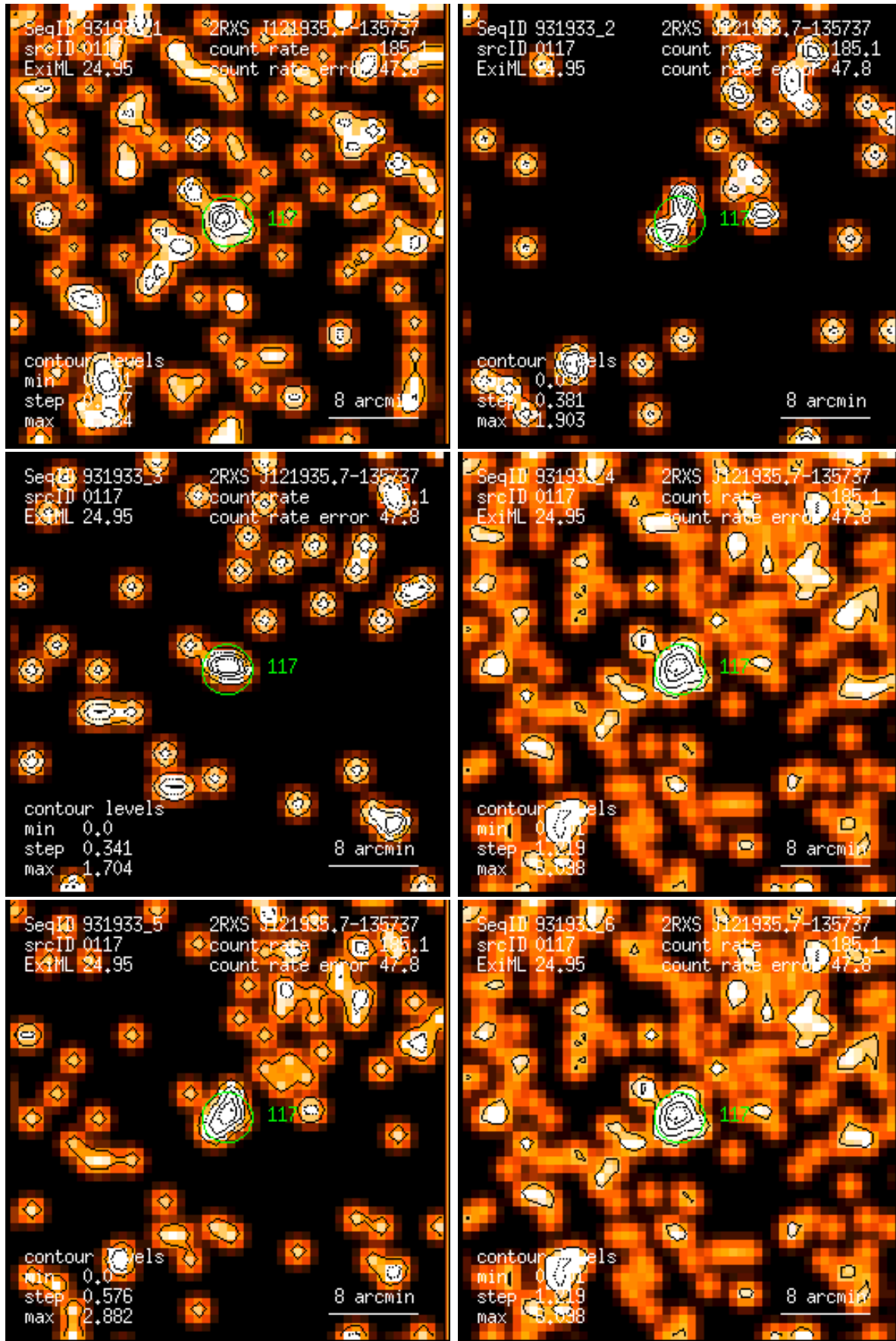
Figure 117: RASS 931933: detection 0117: band rate images, Gaussian filter: (1) PSPC channels 11 – 41, (2) 52 – 90, (3) 91 – 201, (4) 11 – 235, (5) 52 – 201, (6) 11 – 201. Broad band rates in counts/ks. Band rate contour levels in counts/ks/arcmin 2 .
