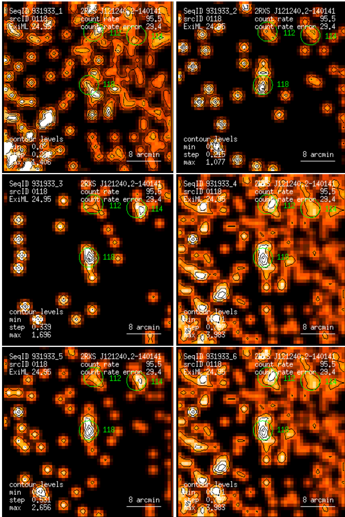
Figure 118: RASS 931933: detection 0118: band rate images, Gaussian filter: (1) PSPC channels 11 – 41, (2) 52 – 90, (3) 91 – 201, (4) 11 – 235, (5) 52 – 201, (6) 11 – 201. Broad band rates in counts/ks. Band rate contour levels in counts/ks/arcmin 2 .
