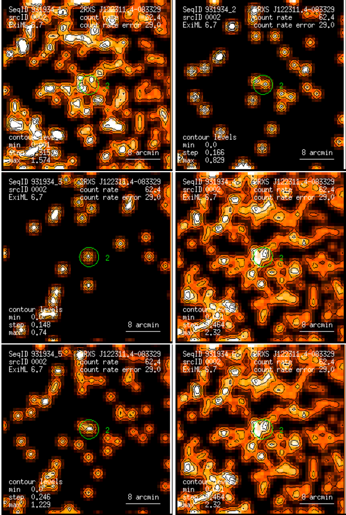
Figure 2: RASS 931934: detection 0002: band rate images, Gaussian filter: (1) PSPC channels 11 – 41, (2) 52 – 90, (3) 91 – 201, (4) 11 – 235, (5) 52 – 201, (6) 11 – 201. Broad band rates in counts/ks. Band rate contour levels in counts/ks/arcmin 2 .
