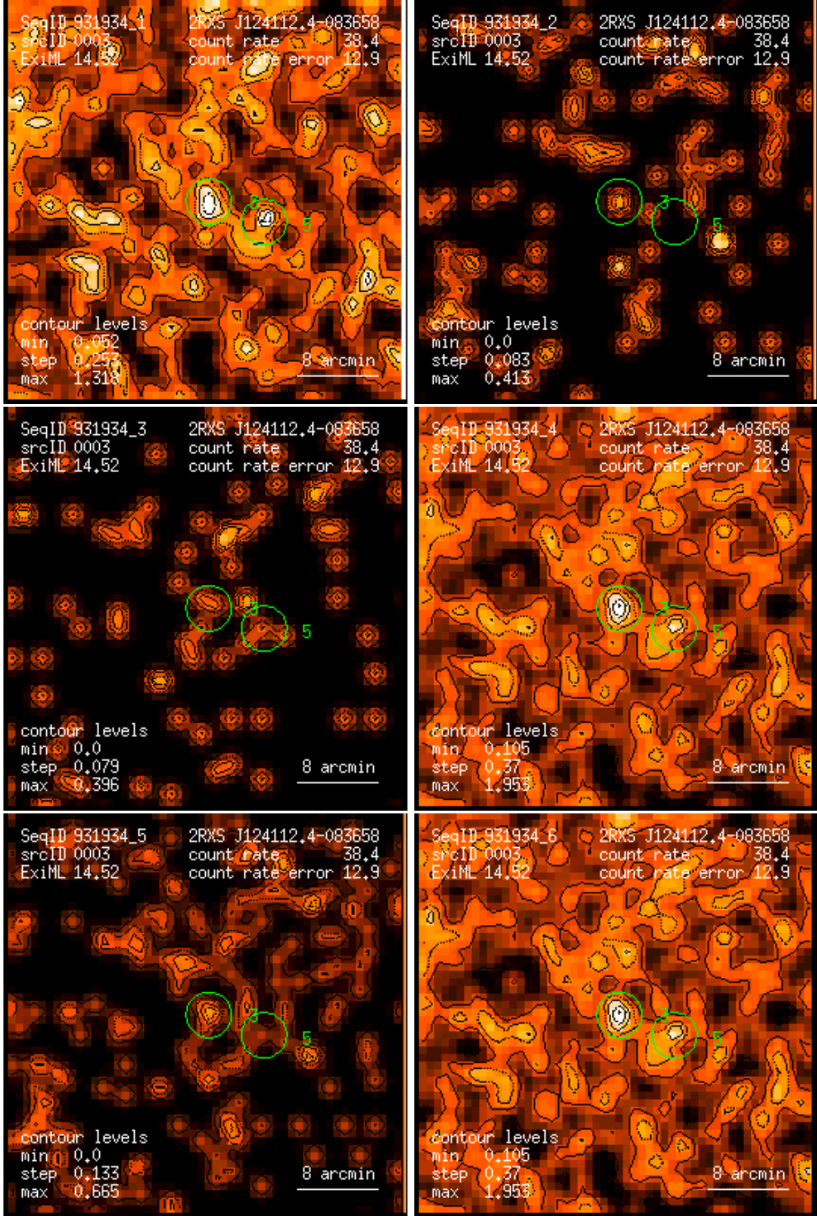
Figure 3: RASS 931934: detection 0003: band rate images, Gaussian filter: (1) PSPC channels 11 – 41, (2) 52 – 90, (3) 91 – 201, (4) 11 – 235, (5) 52 – 201, (6) 11 – 201. Broad band rates in counts/ks. Band rate contour levels in counts/ks/arcmin 2 .
