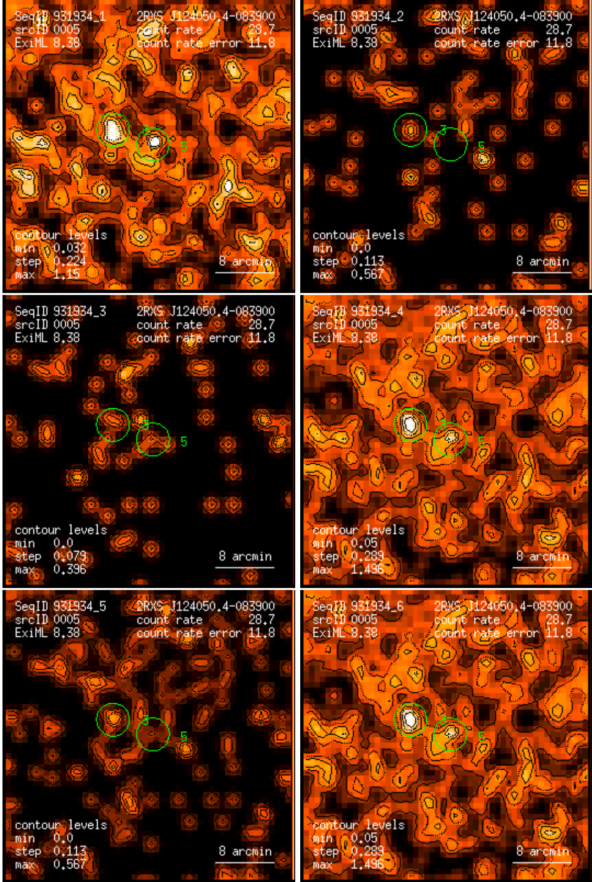
Figure 5: RASS 931934: detection 0005: band rate images, Gaussian filter: (1) PSPC channels 11 – 41, (2) 52 – 90, (3) 91 – 201, (4) 11 – 235, (5) 52 – 201, (6) 11 – 201. Broad band rates in counts/ks. Band rate contour levels in counts/ks/arcmin 2 .
