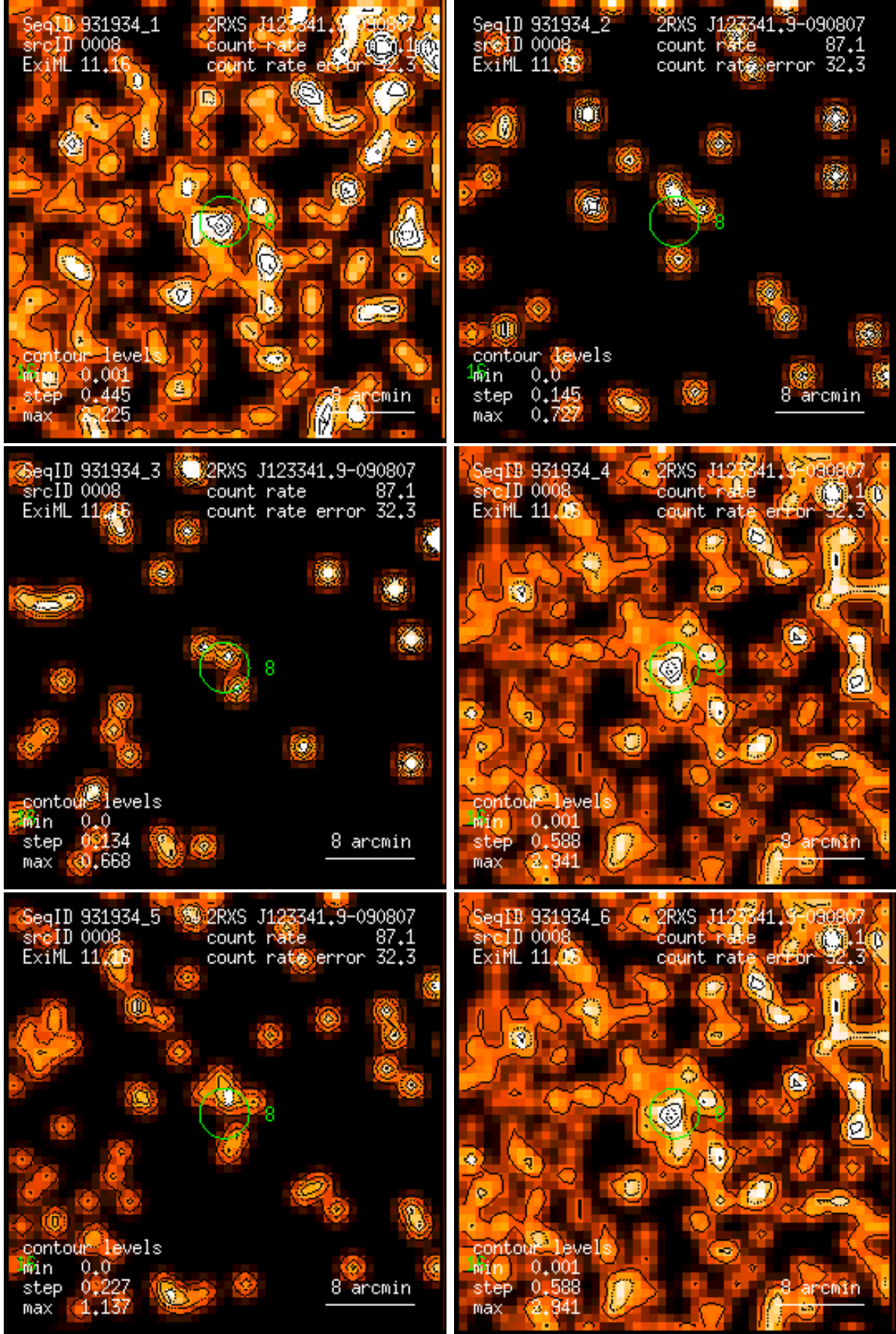
Figure 8: RASS 931934: detection 0008: band rate images, Gaussian filter: (1) PSPC channels 11 – 41, (2) 52 – 90, (3) 91 – 201, (4) 11 – 235, (5) 52 – 201, (6) 11 – 201. Broad band rates in counts/ks. Band rate contour levels in counts/ks/arcmin 2 .
