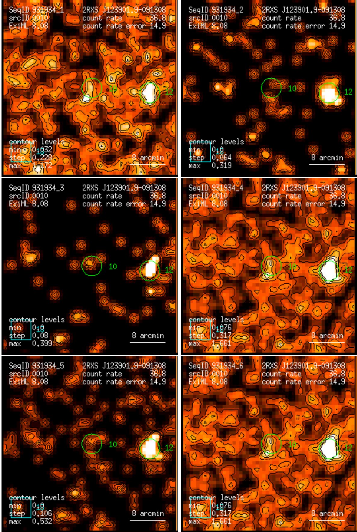
Figure 10: RASS 931934: detection 0010: band rate images, Gaussian filter: (1) PSPC channels 11 – 41, (2) 52 – 90, (3) 91 – 201, (4) 11 – 235, (5) 52 – 201, (6) 11 – 201. Broad band rates in counts/ks. Band rate contour levels in counts/ks/arcmin 2 .
