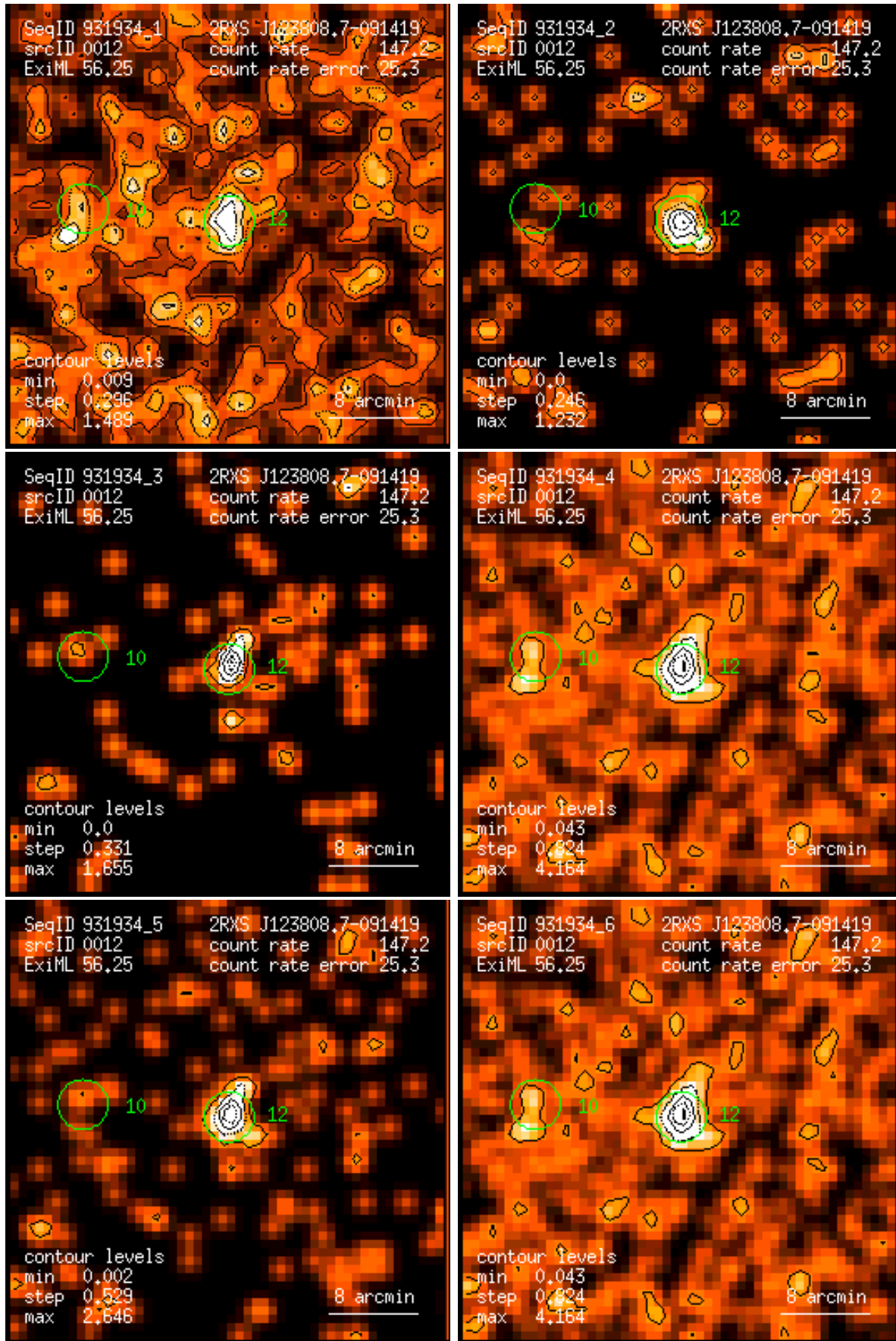
Figure 12: RASS 931934: detection 0012: band rate images, Gaussian filter: (1) PSPC channels 11 – 41, (2) 52 – 90, (3) 91 – 201, (4) 11 – 235, (5) 52 – 201, (6) 11 – 201. Broad band rates in counts/ks. Band rate contour levels in counts/ks/arcmin 2 .
