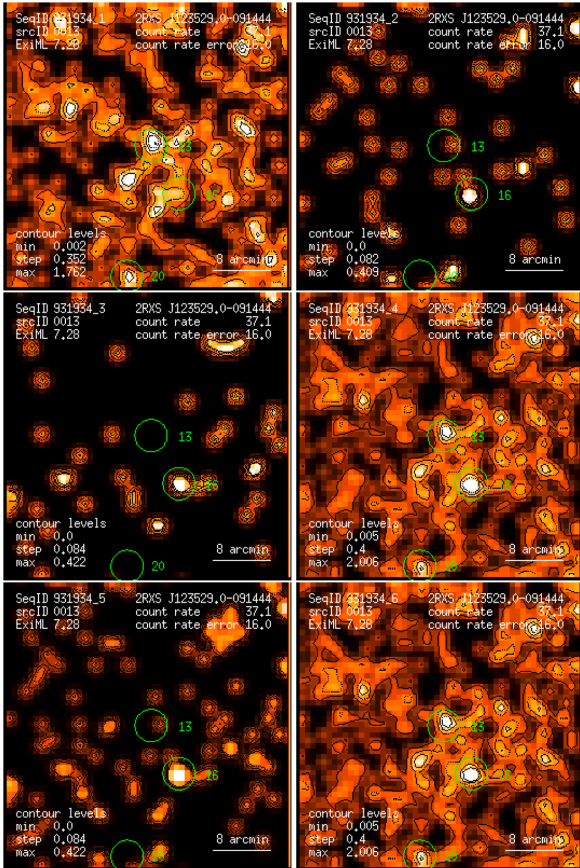
Figure 13: RASS 931934: detection 0013: band rate images, Gaussian filter: (1) PSPC channels 11 – 41, (2) 52 – 90, (3) 91 – 201, (4) 11 – 235, (5) 52 – 201, (6) 11 – 201. Broad band rates in counts/ks. Band rate contour levels in counts/ks/arcmin 2 .
