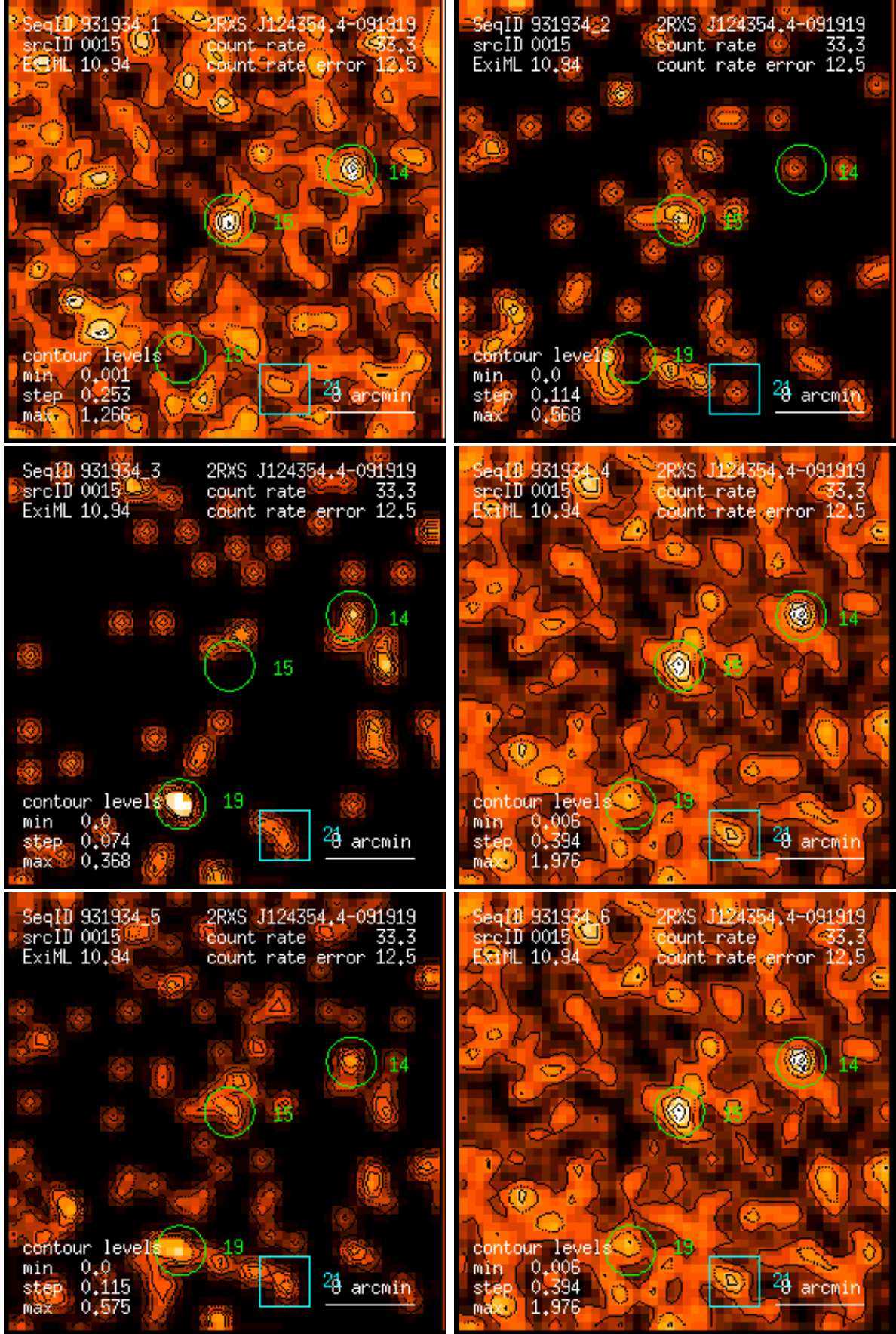
Figure 15: RASS 931934: detection 0015: band rate images, Gaussian filter: (1) PSPC channels 11 – 41, (2) 52 – 90, (3) 91 – 201, (4) 11 – 235, (5) 52 – 201, (6) 11 – 201. Broad band rates in counts/ks. Band rate contour levels in counts/ks/arcmin 2 .
