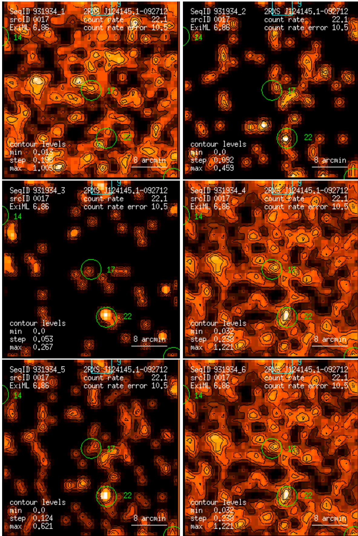
Figure 17: RASS 931934: detection 0017: band rate images, Gaussian filter: (1) PSPC channels 11 – 41, (2) 52 – 90, (3) 91 – 201, (4) 11 – 235, (5) 52 – 201, (6) 11 – 201. Broad band rates in counts/ks. Band rate contour levels in counts/ks/arcmin 2 .
