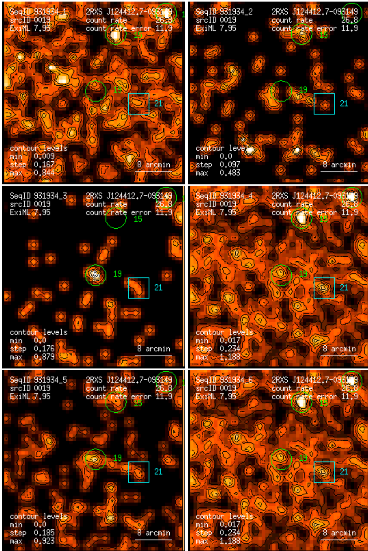
Figure 19: RASS 931934: detection 0019: band rate images, Gaussian filter: (1) PSPC channels 11 – 41, (2) 52 – 90, (3) 91 – 201, (4) 11 – 235, (5) 52 – 201, (6) 11 – 201. Broad band rates in counts/ks. Band rate contour levels in counts/ks/arcmin 2 .
