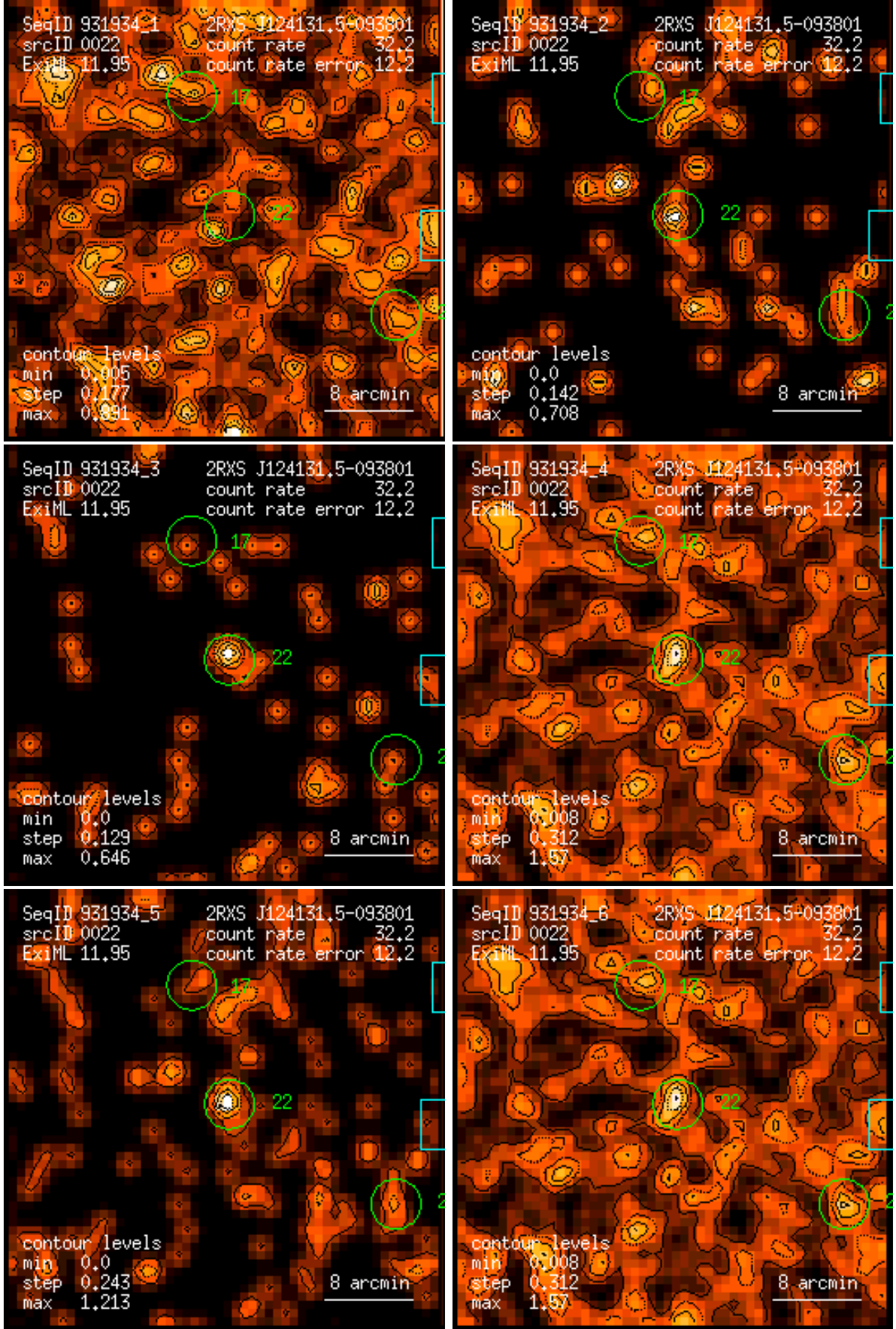
Figure 22: RASS 931934: detection 0022: band rate images, Gaussian filter: (1) PSPC channels 11 – 41, (2) 52 – 90, (3) 91 – 201, (4) 11 – 235, (5) 52 – 201, (6) 11 – 201. Broad band rates in counts/ks. Band rate contour levels in counts/ks/arcmin 2 .
