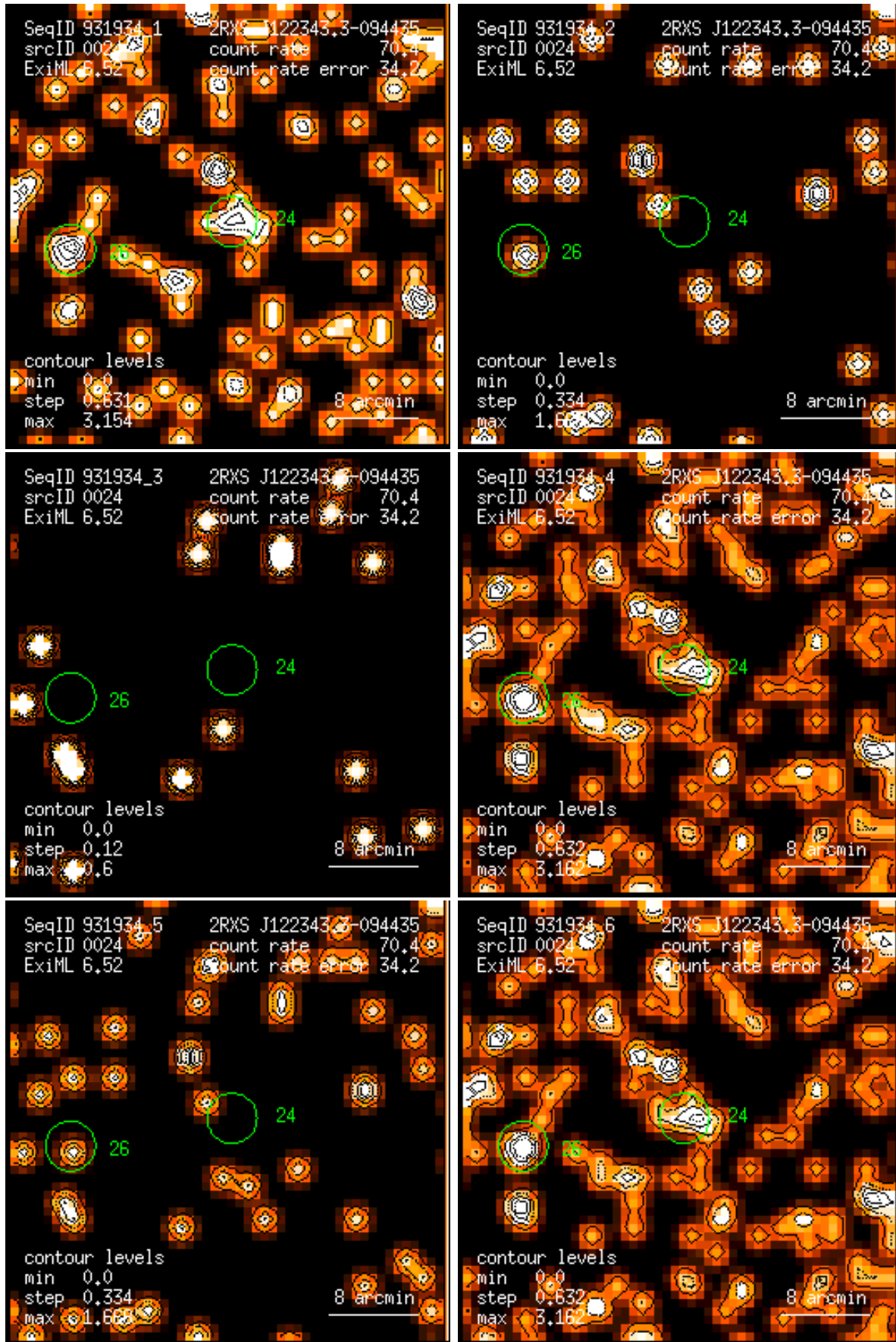
Figure 24: RASS 931934: detection 0024: band rate images, Gaussian filter: (1) PSPC channels 11 – 41, (2) 52 – 90, (3) 91 – 201, (4) 11 – 235, (5) 52 – 201, (6) 11 – 201. Broad band rates in counts/ks. Band rate contour levels in counts/ks/arcmin 2 .
