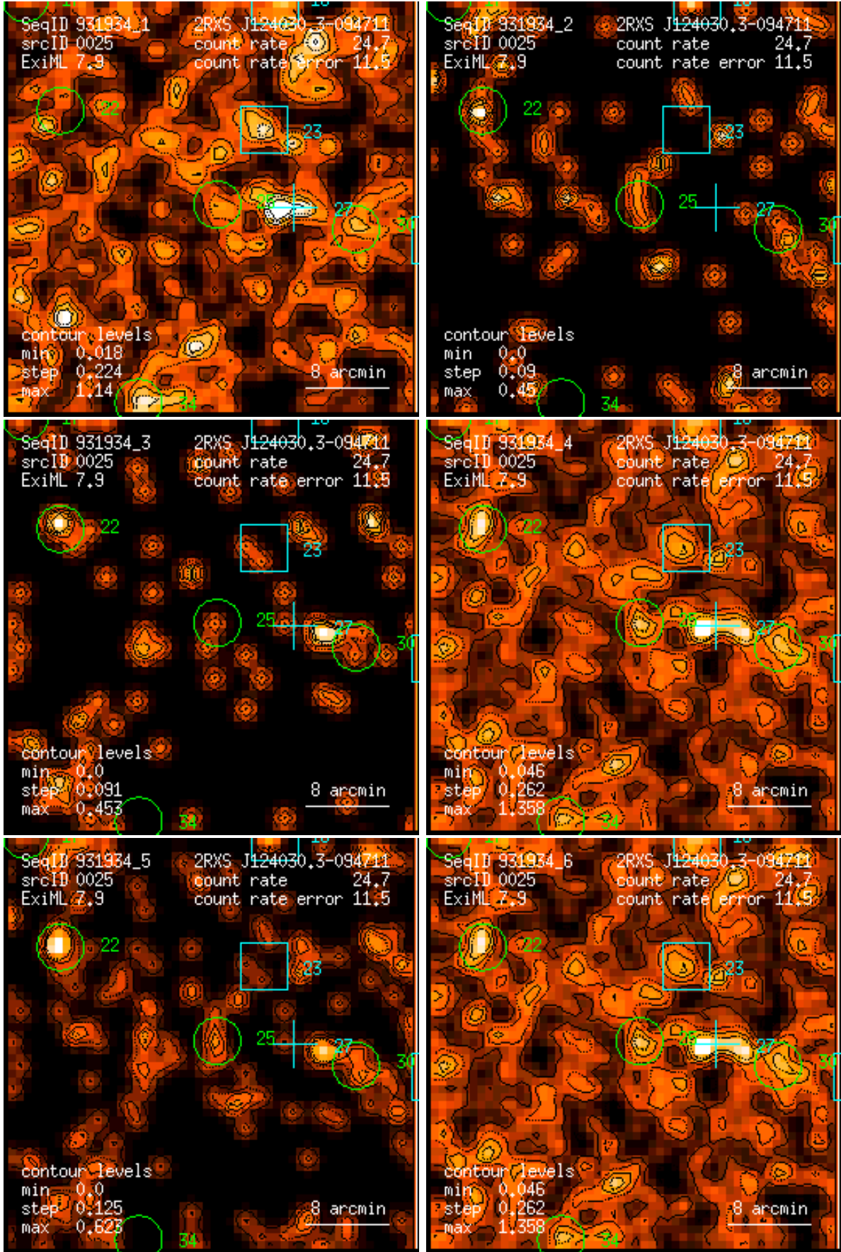
Figure 25: RASS 931934: detection 0025: band rate images, Gaussian filter: (1) PSPC channels 11 – 41, (2) 52 – 90, (3) 91 – 201, (4) 11 – 235, (5) 52 – 201, (6) 11 – 201. Broad band rates in counts/ks. Band rate contour levels in counts/ks/arcmin 2 .
