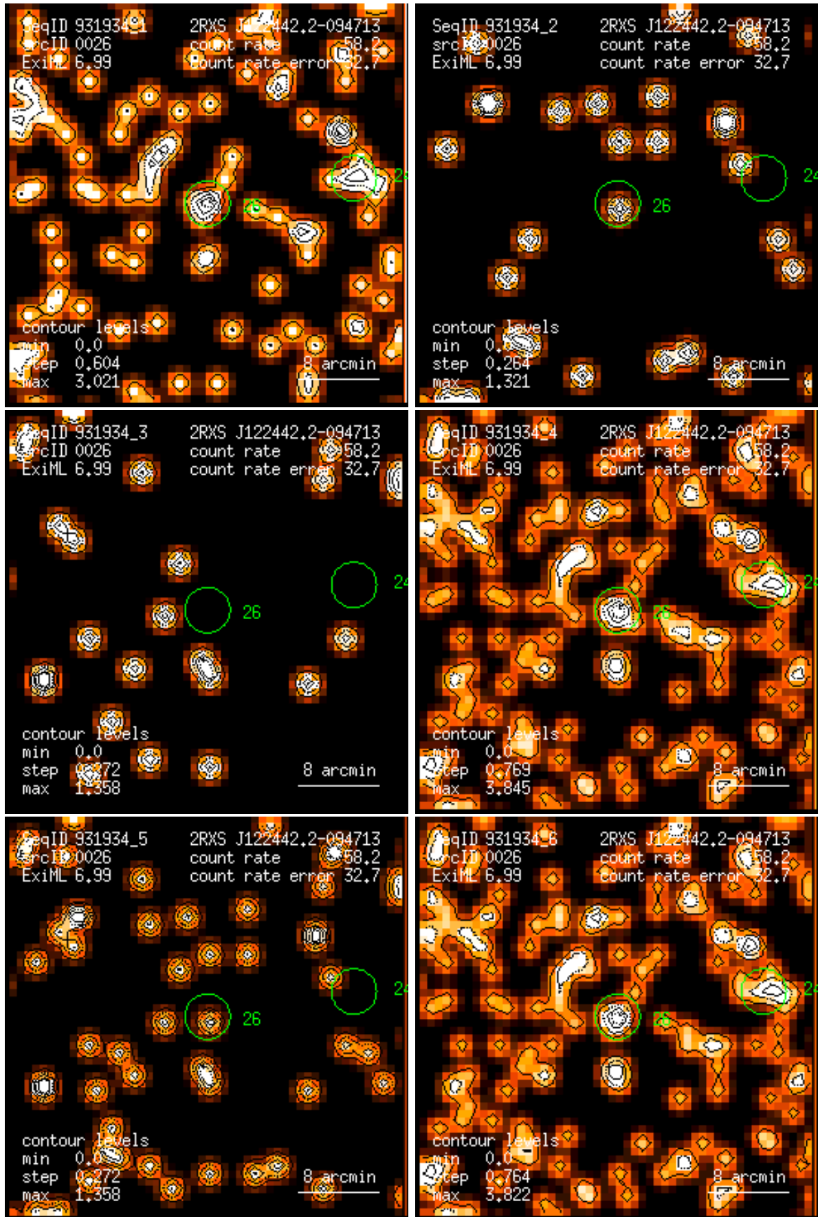
Figure 26: RASS 931934: detection 0026: band rate images, Gaussian filter: (1) PSPC channels 11 – 41, (2) 52 – 90, (3) 91 – 201, (4) 11 – 235, (5) 52 – 201, (6) 11 – 201. Broad band rates in counts/ks. Band rate contour levels in counts/ks/arcmin 2 .
