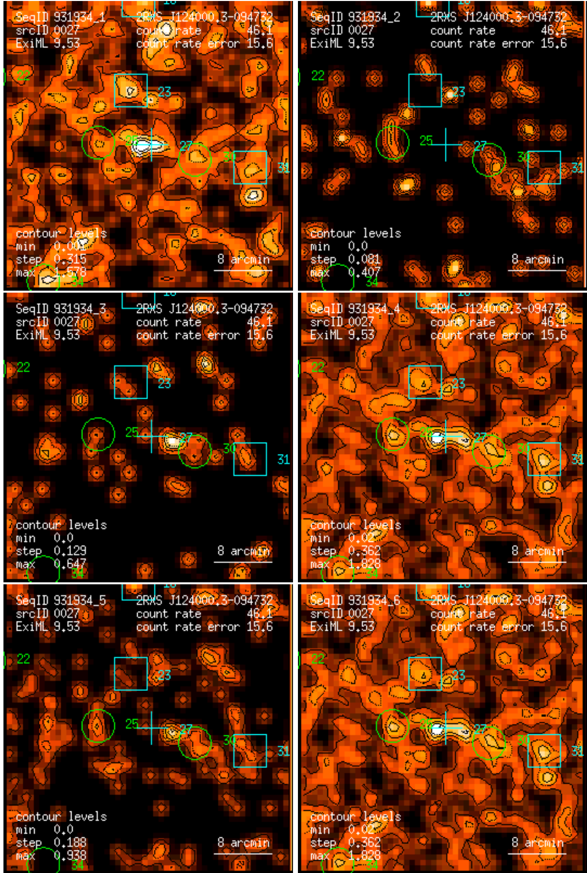
Figure 27: RASS 931934: detection 0027: band rate images, Gaussian filter: (1) PSPC channels 11 – 41, (2) 52 – 90, (3) 91 – 201, (4) 11 – 235, (5) 52 – 201, (6) 11 – 201. Broad band rates in counts/ks. Band rate contour levels in counts/ks/arcmin 2 .
