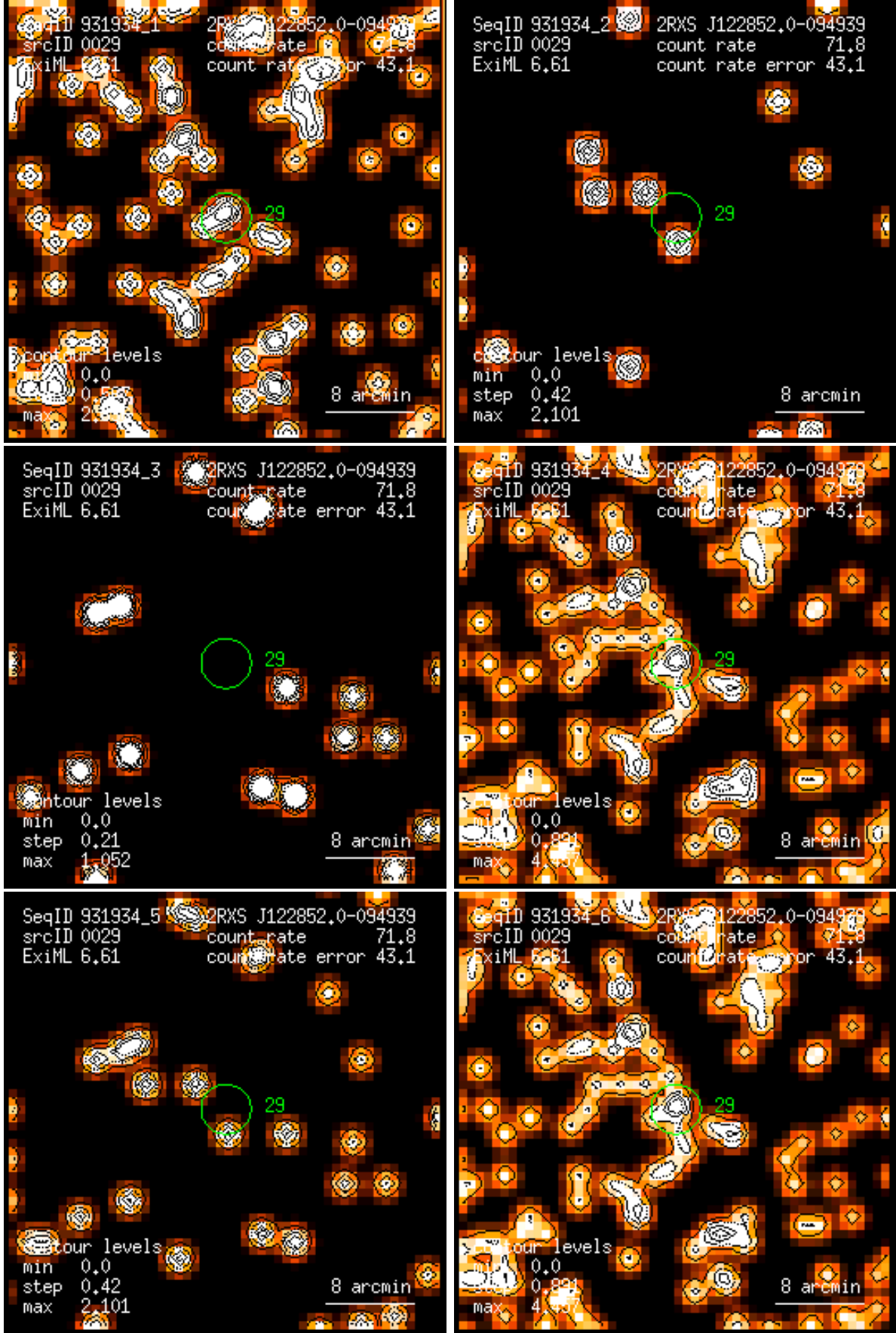
Figure 29: RASS 931934: detection 0029: band rate images, Gaussian filter: (1) PSPC channels 11 – 41, (2) 52 – 90, (3) 91 – 201, (4) 11 – 235, (5) 52 – 201, (6) 11 – 201. Broad band rates in counts/ks. Band rate contour levels in counts/ks/arcmin 2 .
