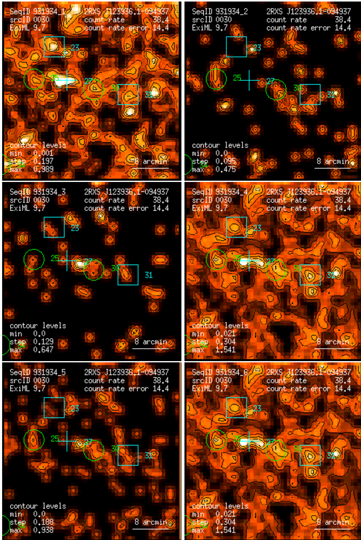
Figure 30: RASS 931934: detection 0030: band rate images, Gaussian filter: (1) PSPC channels 11 – 41, (2) 52 – 90, (3) 91 – 201, (4) 11 – 235, (5) 52 – 201, (6) 11 – 201. Broad band rates in counts/ks. Band rate contour levels in counts/ks/arcmin 2 .
